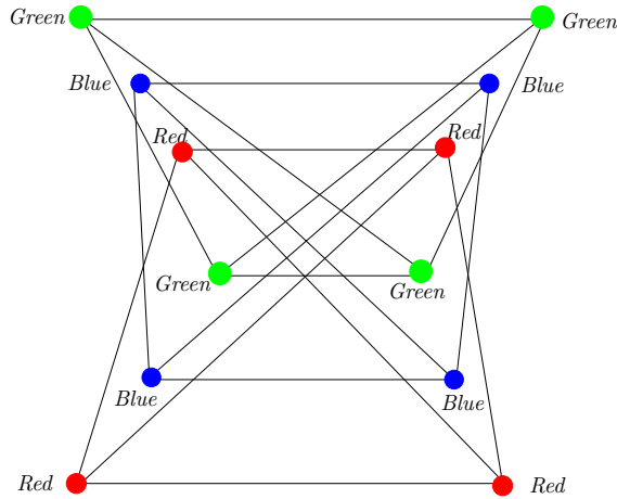
FIGURE 1. A set of 3-colored 12 points that does not contain any monochromatic triangle with at most 1 interior point.
