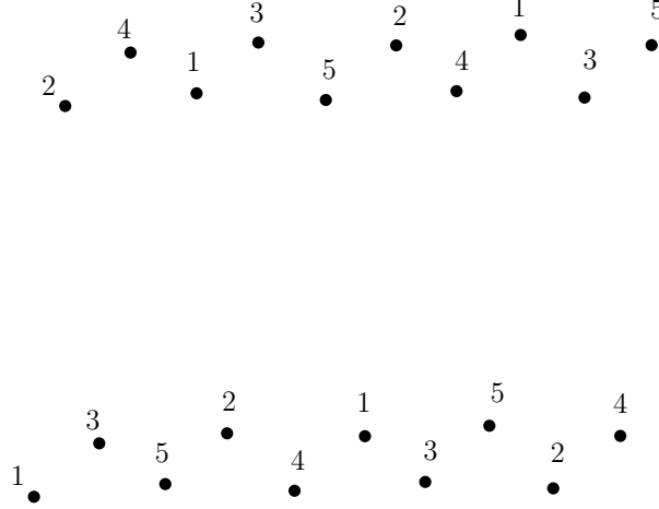
FIGURE 2. A Horton set colored with 5 colors. The number next to a point denotes the color of the point. Observe that the coloring splits in a cyclical manner in H^+ and H^- .
