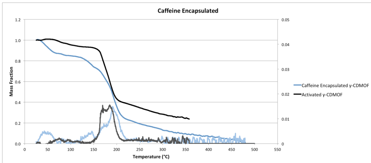
Figure 13. Thermograms with derivation curves of the caffeine encapsulated sample and the as-activated sample
