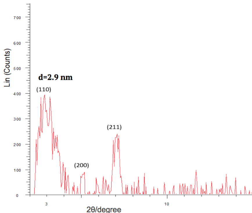
Figure 10. XRD diffractogram of the as-activated \gamma -CDMOFs showing three distinct peaks associated with different crystal planes
