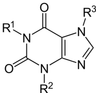
Figure 3. The general chemical structure for xanthine and the two methylxanthines [24]
