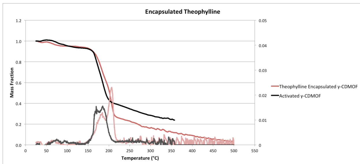
Figure 12. Thermograms with derivation curves of the theophylline-encapsulated sample and the as-activated sample
