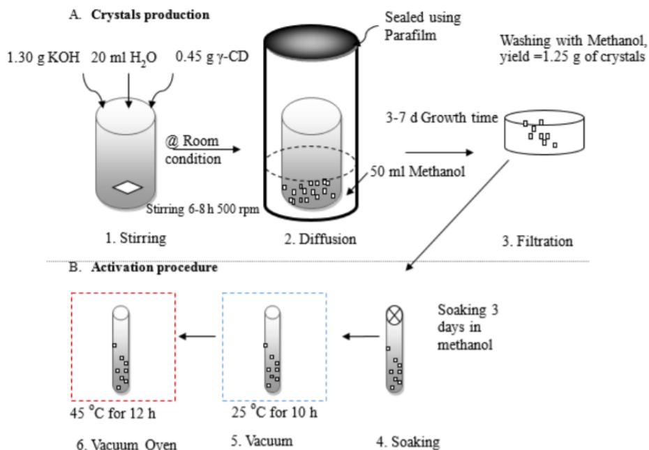
Figure 5. The growth and activation procedure for \gamma -CDMOFs [29]
