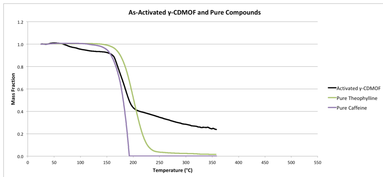
Figure 11. Thermograms of the as-activated \gamma -CDMOF, pure theophylline, and pure caffeine
