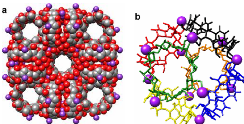
Figure 2. a) Space-filled depiction of solid state extended structure of CDMOFs where grey represents carbon, red represents oxygen, and purple represents potassium; b) Representation of \gamma -CD with K^+ cations (purple) coordinated to primary and secondary faces [12]
