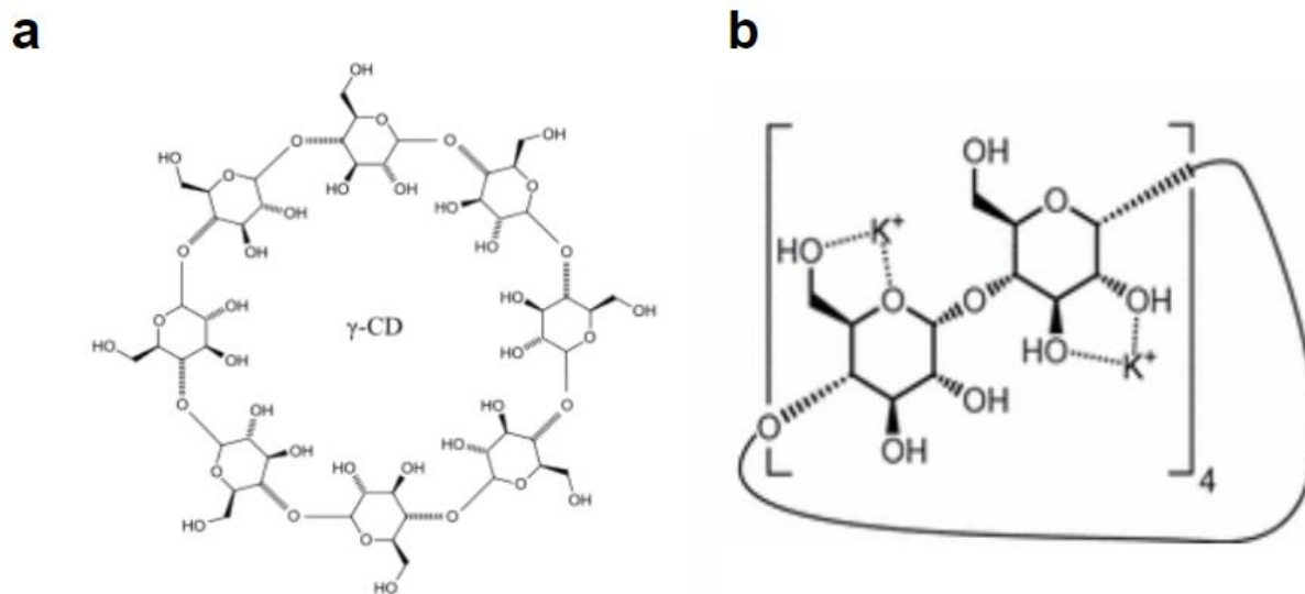
Figure 1. a) Chemical structure of \gamma -CD [11]; b) Structural formula of CDMOFs, depicting coordination of K^+ cations [12]
