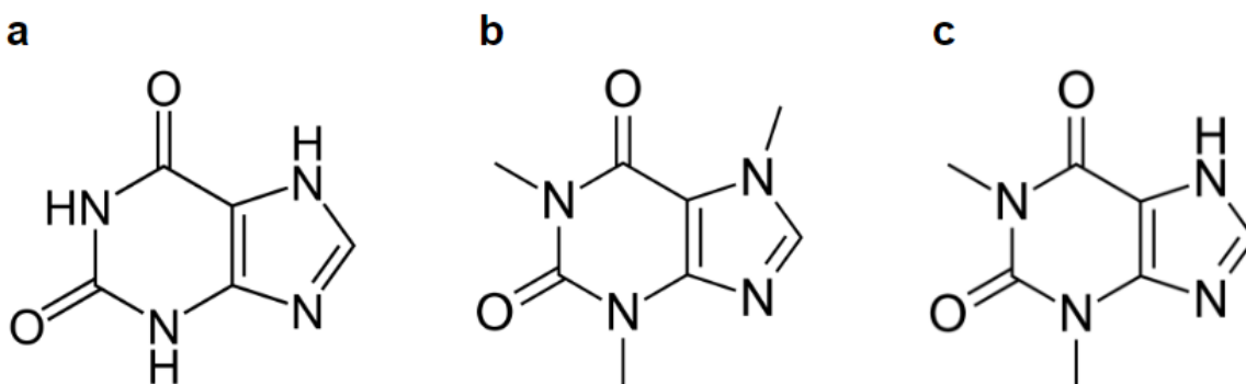
Figure 4. The chemical structure of the xanthine and the two methylxanthines. a) xanthine; b) caffeine; c). theophylline [25],[26],[27]
