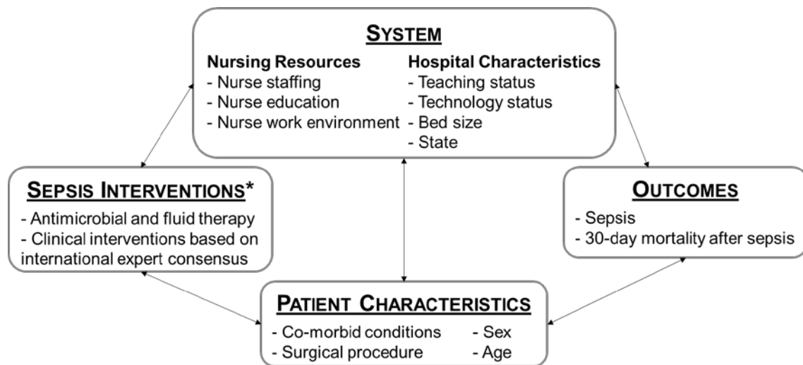
FIGURE 2.1: Conceptual Model
