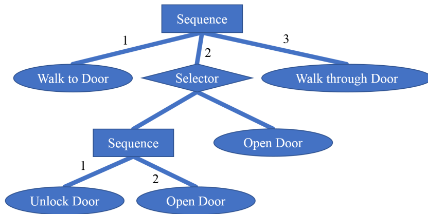
Figure 2.1: Example of a behavior tree for generating NPC behavior.
