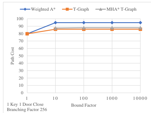
Figure 7.11: Performance results for 1 Key 1 Door Close scenario.
