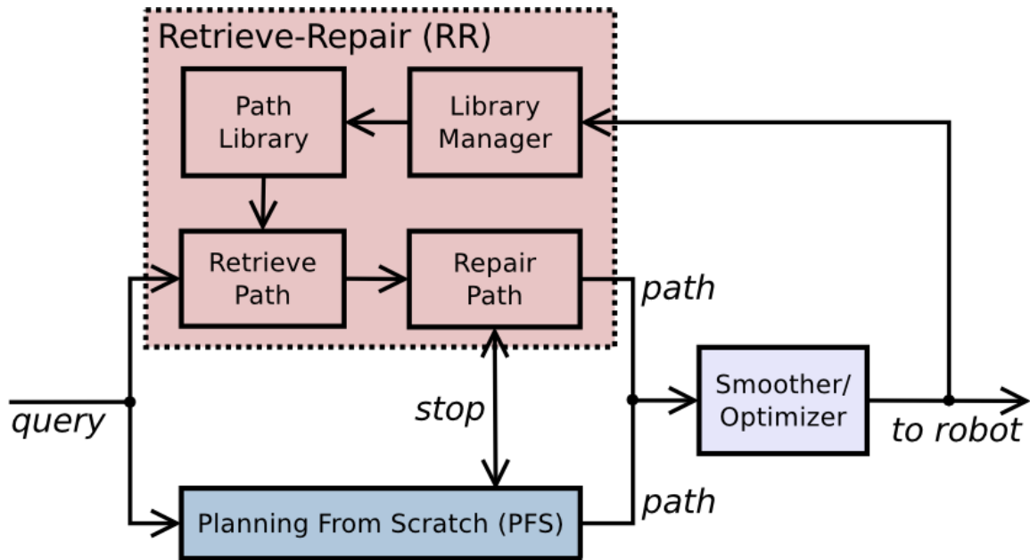
Figure 2.5: Lightning system diagram, from [42]
