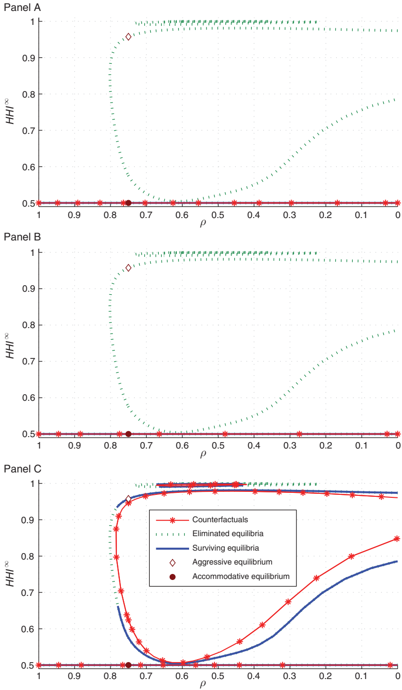
FIGURE 3. COUNTERFACTUAL AND EQUILIBRIUM CORRESPONDENCES
