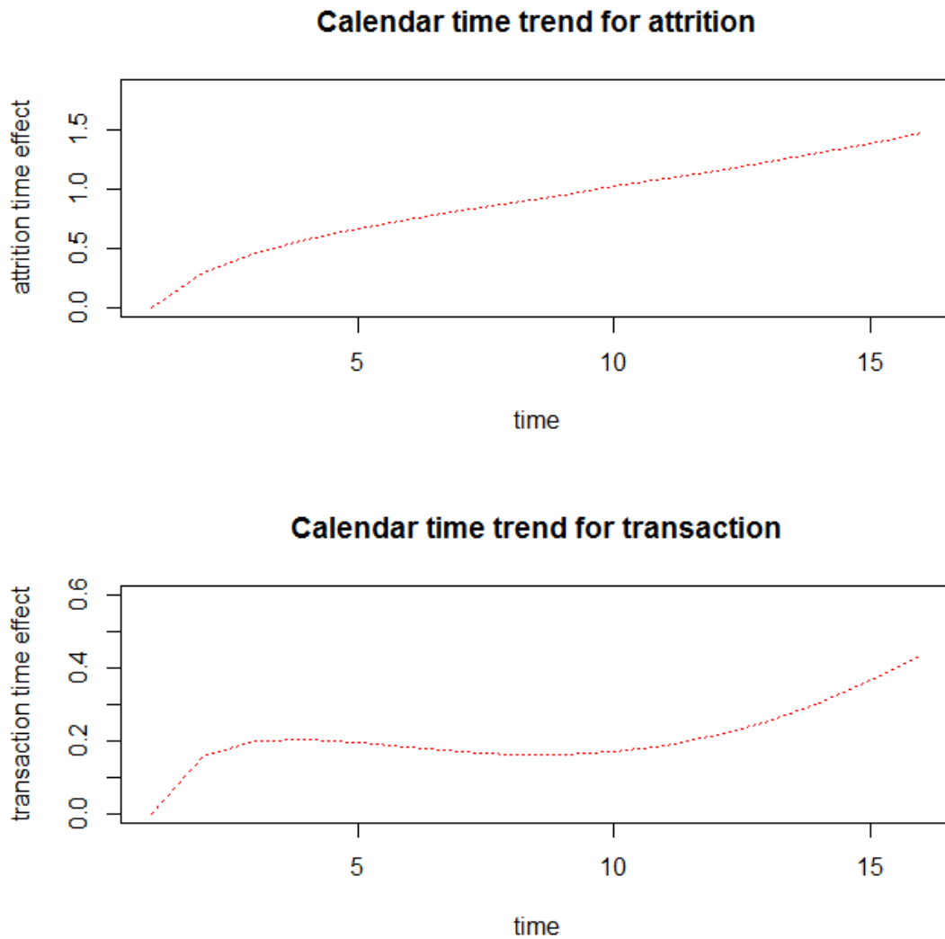
Figure D-1: Simulated calendar-time effects for attrition and transaction processes. Only the first 12 time periods are covered in the in-sample data.
