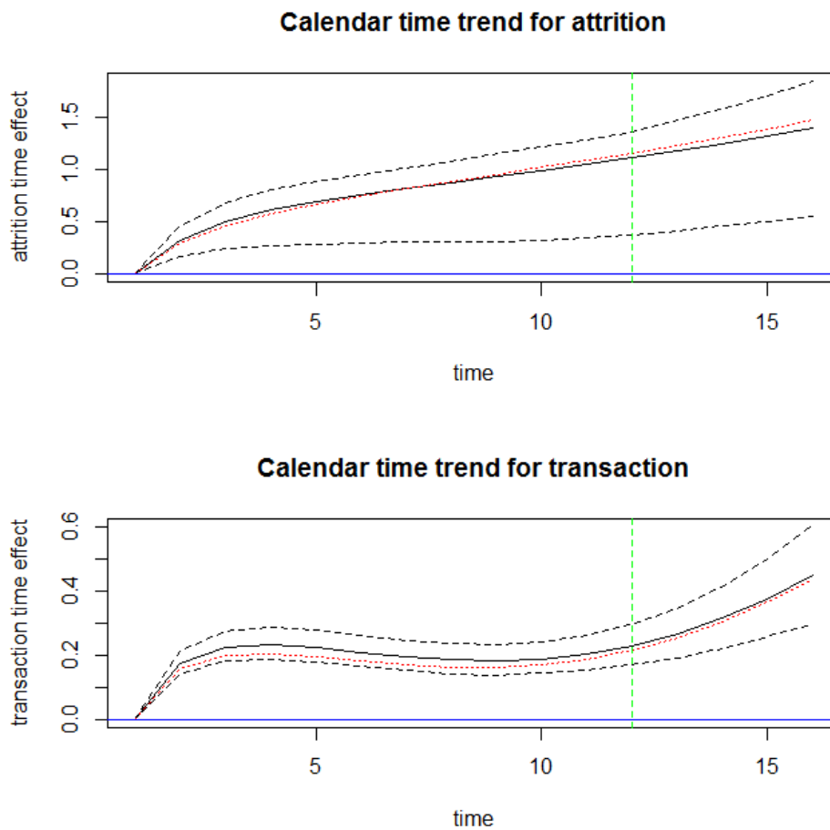
Figure D-2: Recovered calendar-time effects. Solid line is the posterior median time effect. Large-dash dotted lines represent the 95% posterior interval for the time effect. Small-dash dotted lines represent the true calendar-time effect. Vertical line shows in-sample cutoff.
