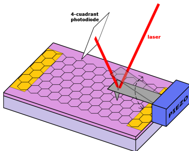
Figure 3.3: Diagram of AFM operation. Piezoelectric sensor controls the oscillation, movement in the horizontal plane and the height. A feedback loop keeps the measured force constant.
