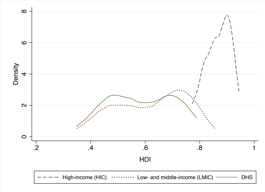
Figure A1 Kernel density of countries over Human Development Index (HDI), by group of countries
