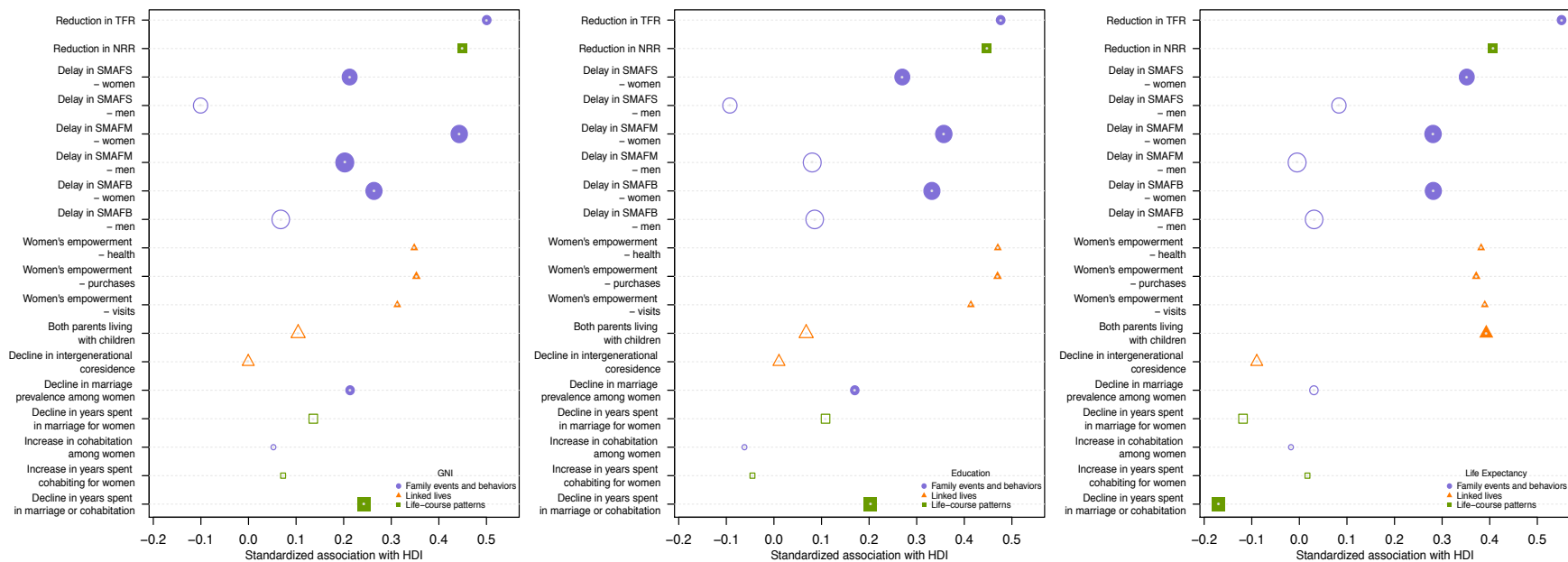
Figure A4 Associations between HDI-components and GFC-indicators, global analysis. GNI (left), education (center), and life expectancy (right)
