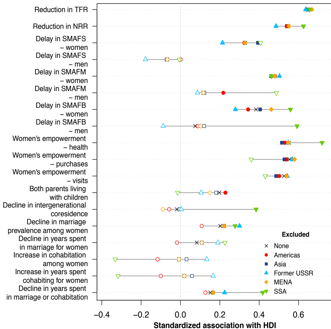
Figure 5 Associations between HDI and GFC-indicators, regional analysis
