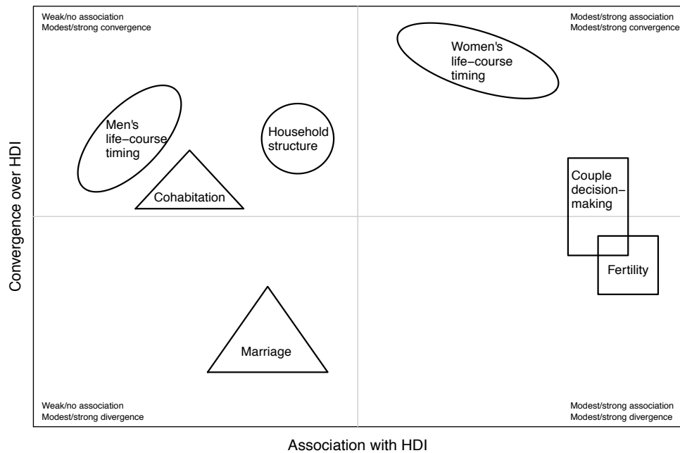
Figure 1 Framework of analysis and general overview of findings
