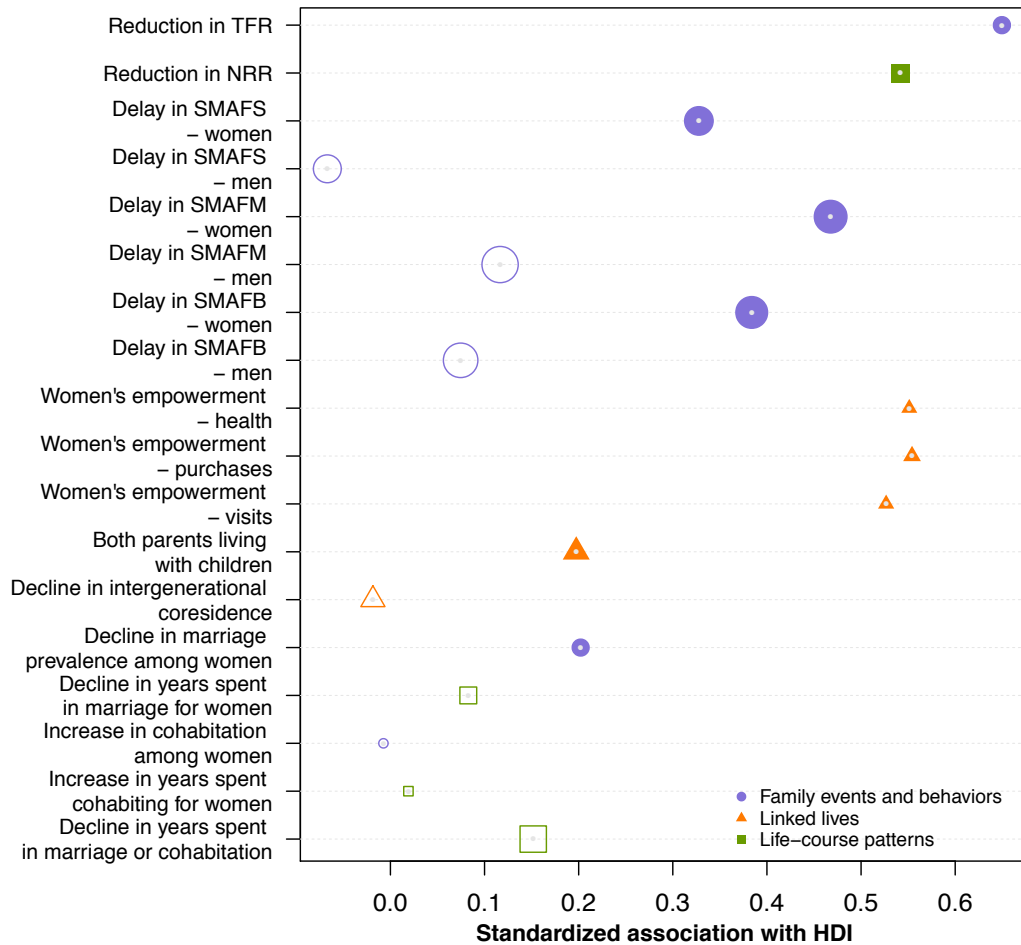
Figure 4 Associations between HDI and GFC-indicators, global analysis
