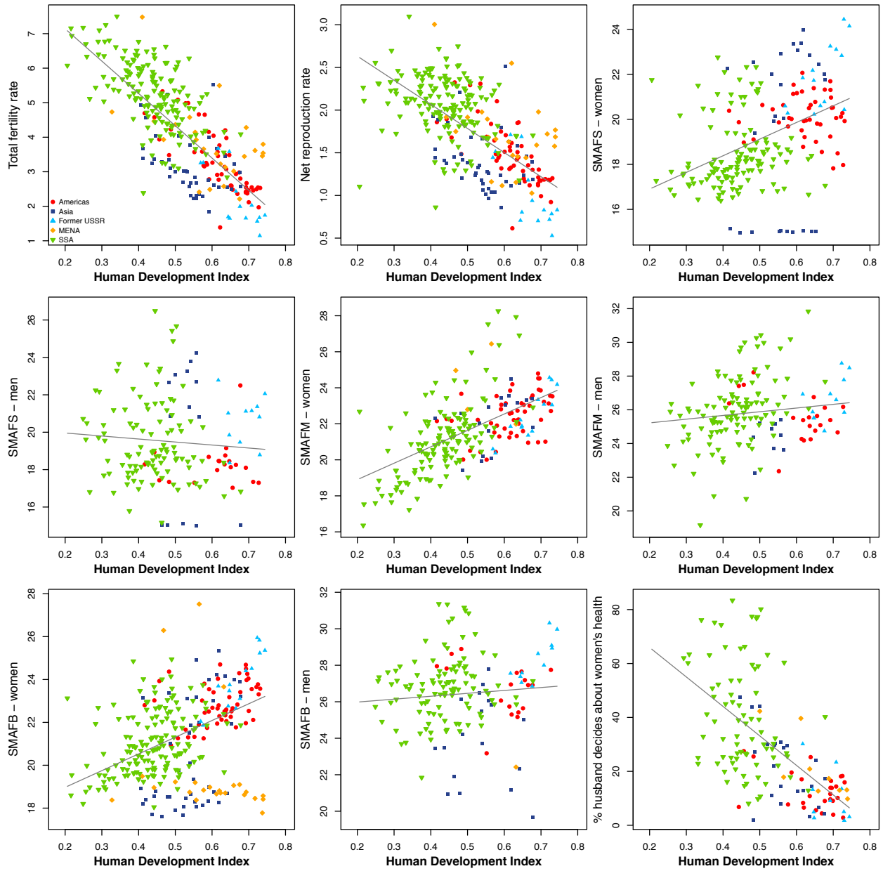
Figure A3 Scatter plots of the association between GFC-indicators and HDI
