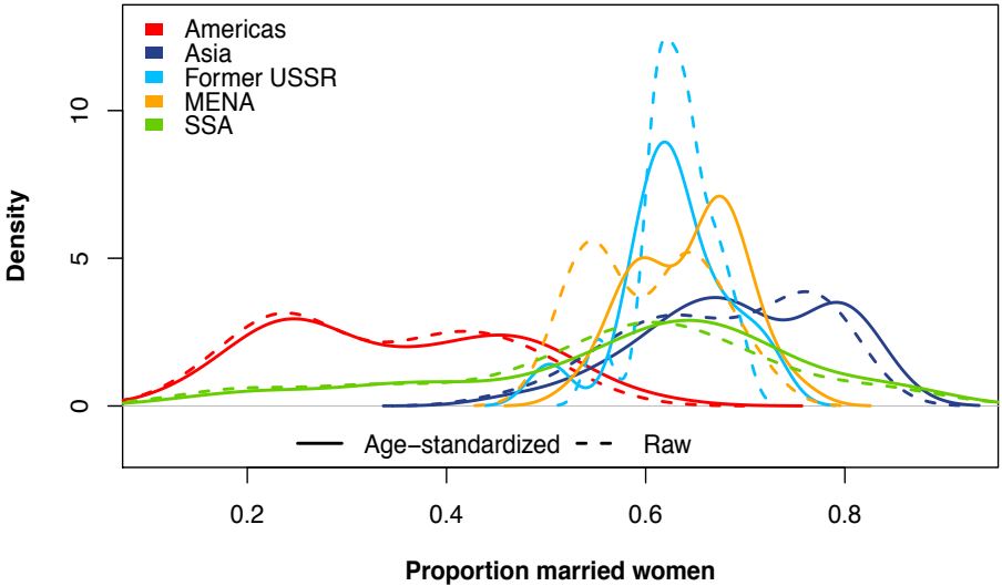
Figure A2 Age-standardized vs crude family indicators. Example shown: age-standardized vs crude marriage prevalence
