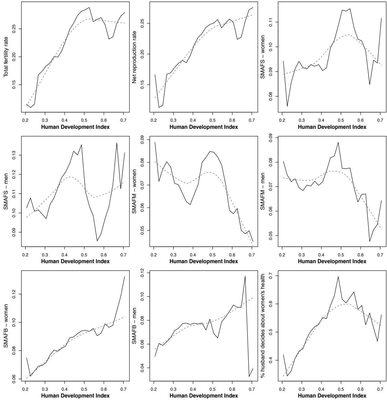
Figure A5 Sigma-convergence over HDI
