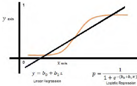
FIGURE 5. Logistic regression.
