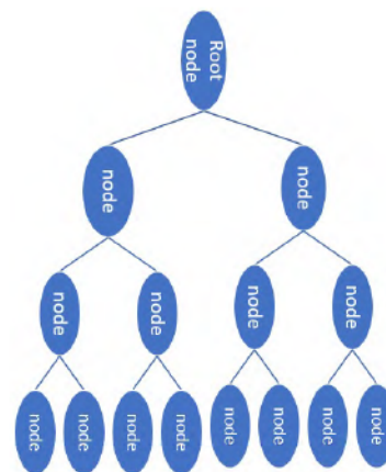
FIGURE 4. Decision tree.
