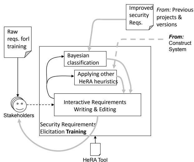
Fig. 12 A stakeholder trains security requirements elicitation.
