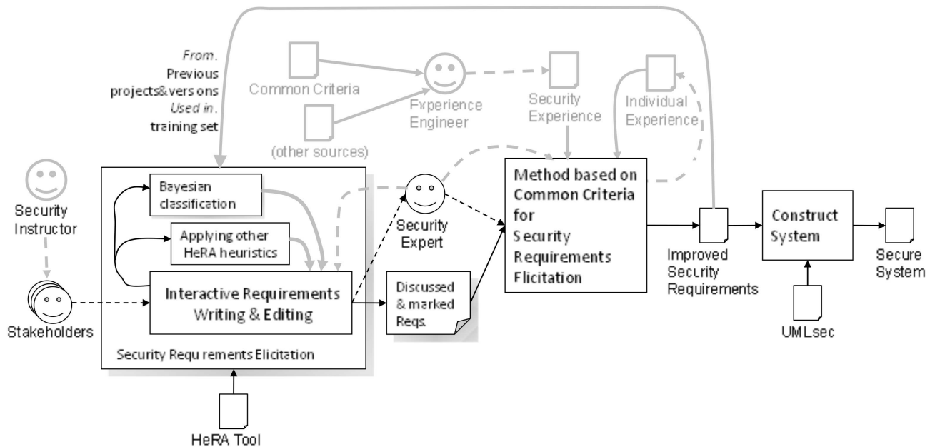
Fig. 9 Overview of SecReq approach with solid feedback from UMLsec to HeRA. In this model, Security Requirements Elicitation is supported by applying Bayesian classifiers. They are trained by reusing documents from earlier projects. Specifications from previous projects are used to train the classifiers. This establishes a solid feedback.
