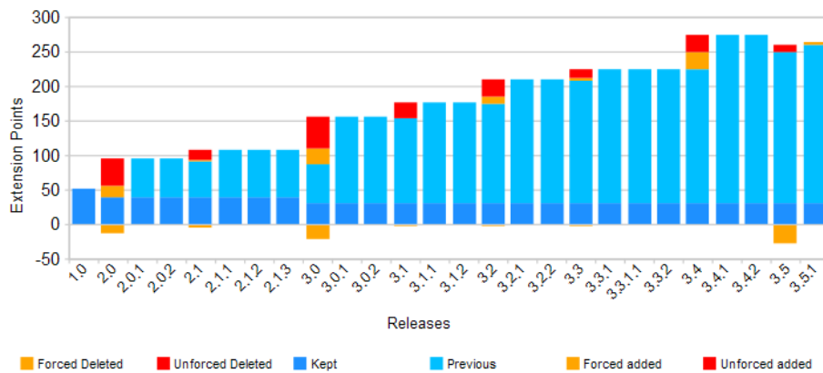
Fig. 8 Evolution of the absolute number of extension points
