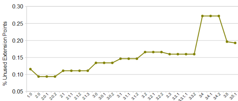
Fig. 11 Evolution of the percentage of unused extension points
