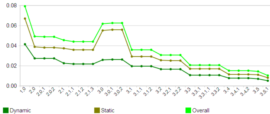
Fig. 6 Evolution of the cohesion
