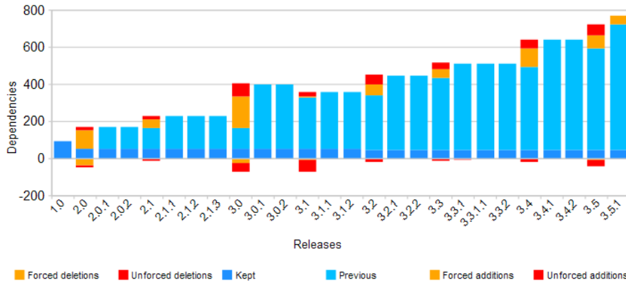
Fig. 5 Evolution of the overall complexity
