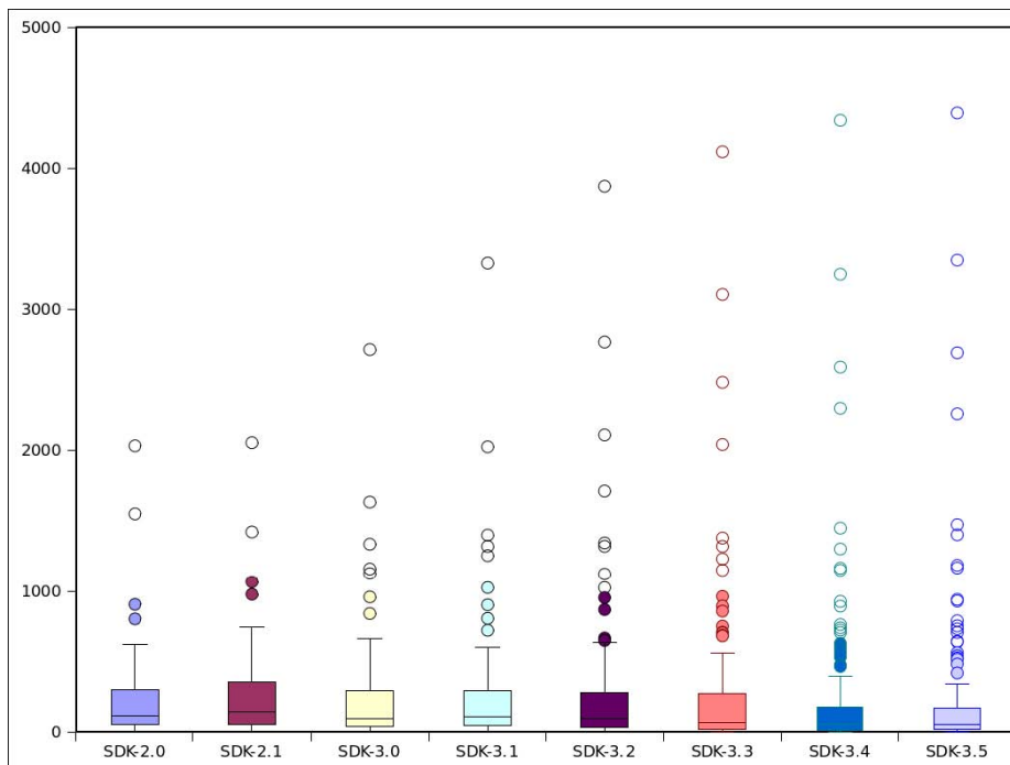
Fig. 16 Evolution of the number of classes per plugin
