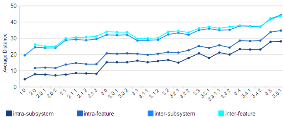
Fig. 14 Evolution of the average intra- and inter-unit distance in CCVisu's graphs
