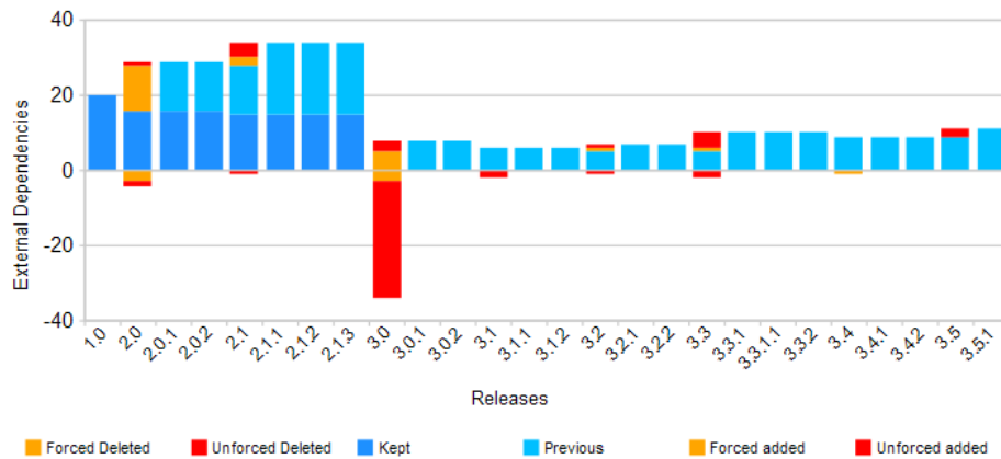
Fig. 7 Evolution of the coupling
