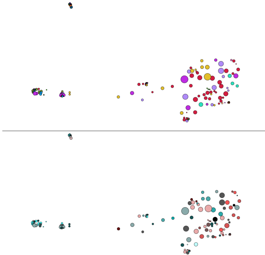
Fig. 15 Assessing the CCP, over all releases, for features (top) and subsystems (bottom)
