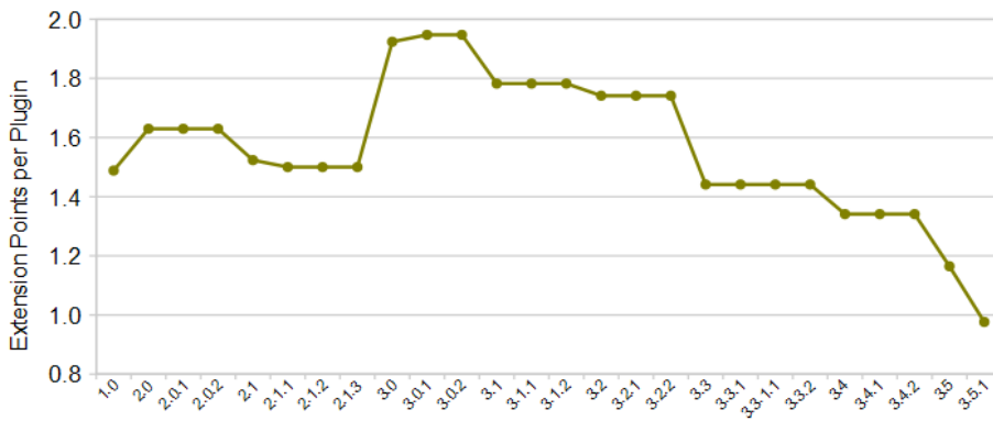
Fig. 9 Evolution of the plugin to extension point ratio
