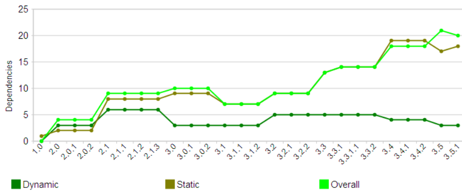
Fig. 12 Evolution of the number of dependencies violating the SDP
