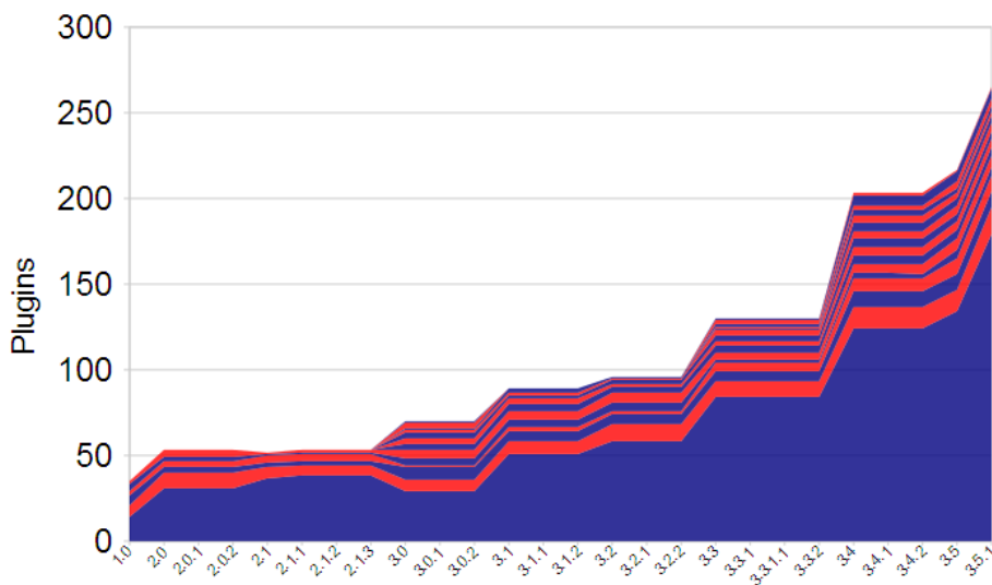
Fig. 2 Evolution of the architecture's layers
