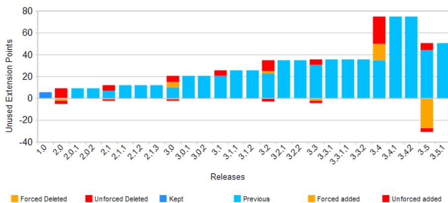
Fig. 10 Evolution of the absolute number of unused extension points
