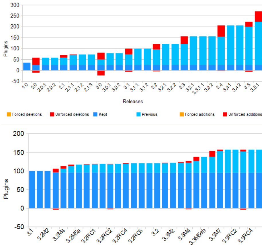
Fig. 4 Evolution of the size
