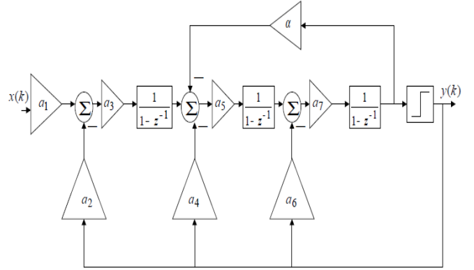
Fig. 4. \Delta - \Sigma demodulator.
