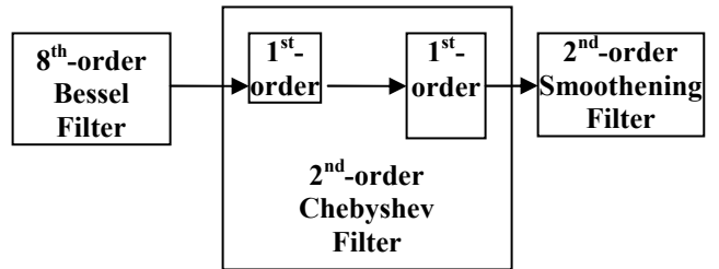
Fig. 5. On-chip analog filtering.
