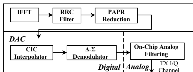
Fig. 1. Baseband transmitter architecture.
