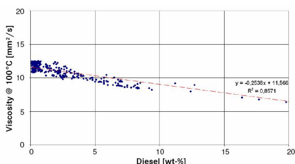
Figure 3.1.: Effect of oil dilution by Diesel fuel on kinematic viscosity
