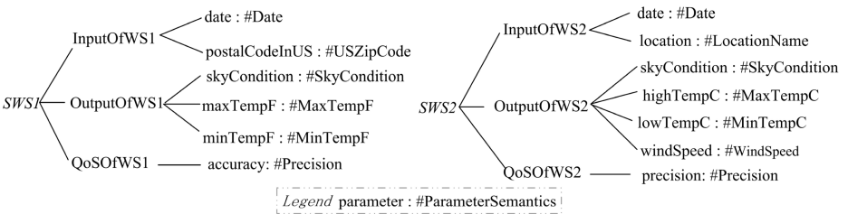
Fig. 4. Examples of semantic Web services
