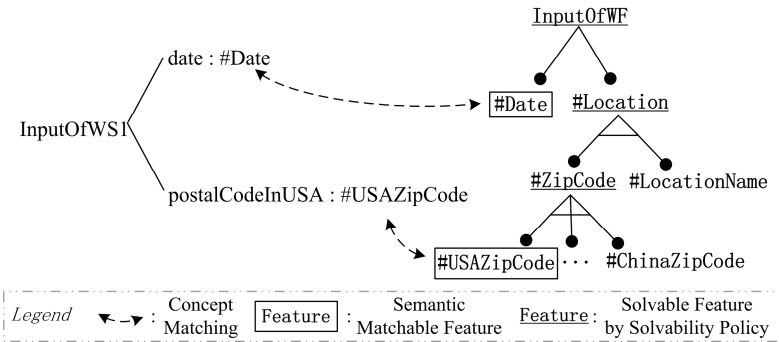
Fig. 5. Example of service matching between domain services and semantic Web services
