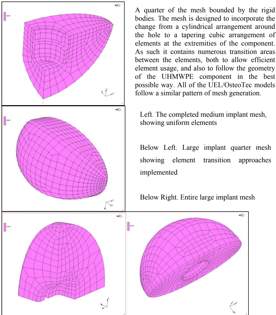
Fig 6 FEA analysis of the articulating surfaces of the UEL/ OsteoTec wrist prosthesis
