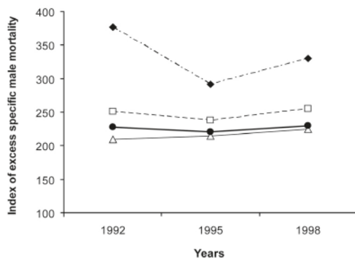
Figure 1. Index of excess specific mortality of men in Slovenia for the studied years for different age groups. Age-specific mortality of women equals 100. Symbols and lines denote age groups: closed diamonds with dash-dot line – 25-34 y; open squares with dashed line – 35-44 y; open triangles with thin solid line – 45-54 y; closed circles with thick solid line – 55-64 y.
