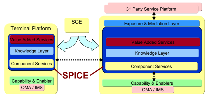
Fig. 9. Layers in the SPICE Architecture
