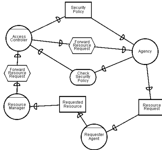
Figure 6: The ACCESS CONTROLLER Dependencies
