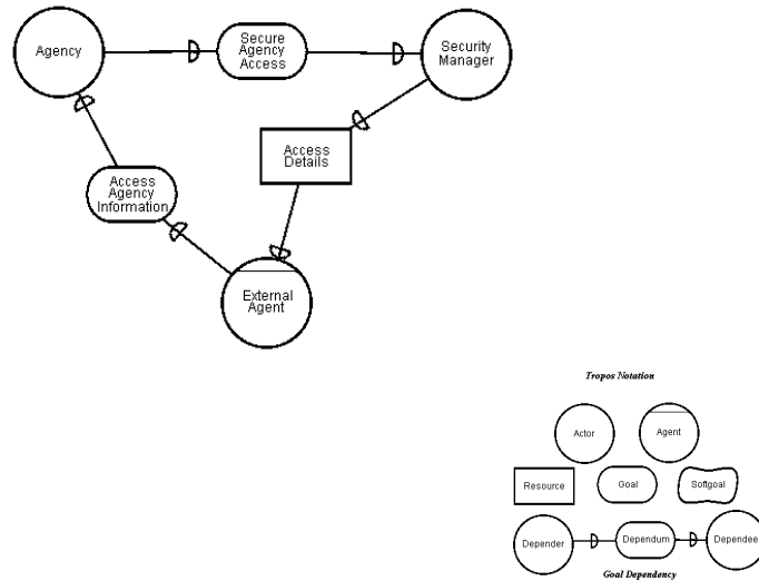
Figure 1: An example of representing social dependencies between different actors of the system
