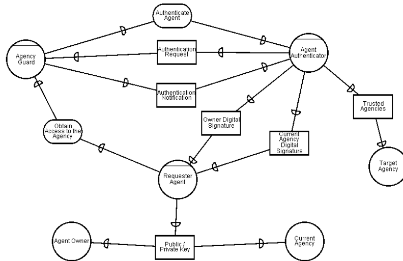
Figure 4: The AGENT AUTHENTICATOR Dependencies
