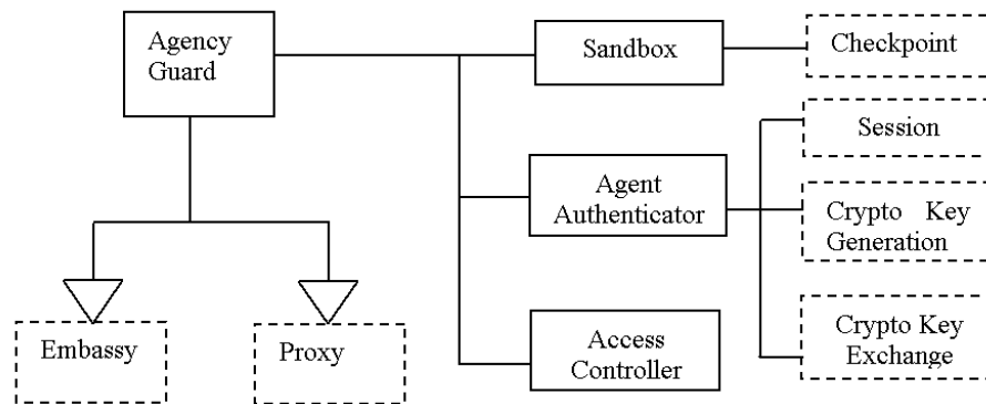
Figure 2: Patterns Roadmap
