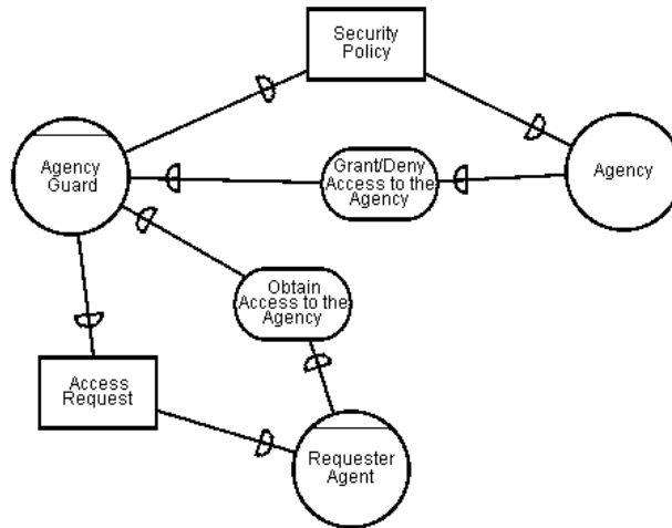
Figure 3: The AGENCY GUARD Dependencies
