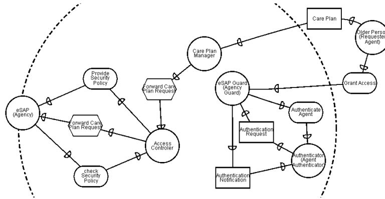
Figure 7: An example of using the patterns
