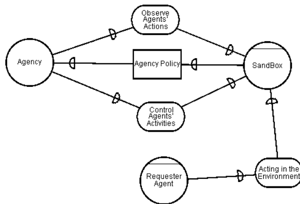
Figure 5: The SANDBOX Dependencies
