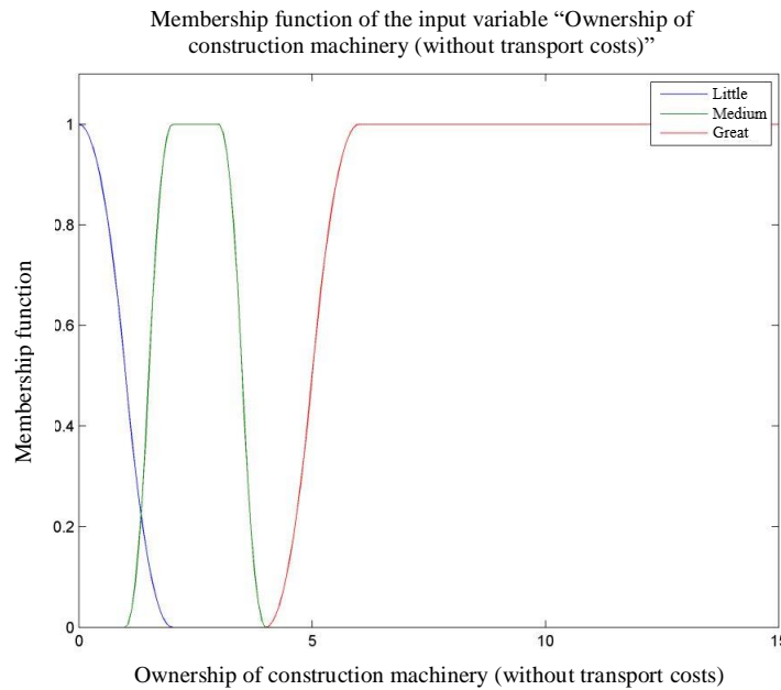
Figure 7. Membership function of the input variable “Ownership of construction machinery (without transport costs)”.
