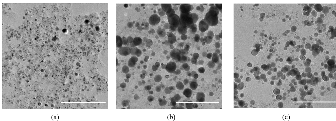
Figure 8. TEM images of pyrolyzed bulk samples of (a) PM3 , (b) PM5 and (c) 4 (scale bar = 200 nm).
