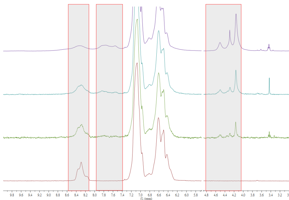
Figure 2. ^1\text{H} NMR spectra of PM2 with x = 0, 0.1, 0.2 and 0.4 from the bottom to the top in \text{CD}_2\text{Cl}_2 .
