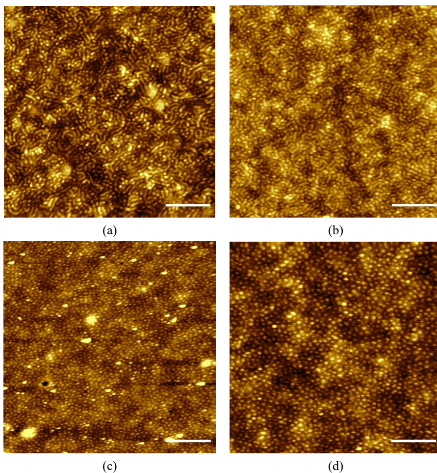
Figure 6. AFM height images of as-spun (a) PM1 , (b) PM2 , (c) PM3 and (d) PM4 with a ca. 20 % loading of complex 3 on silicon wafers (scale bar: 400 nm).
