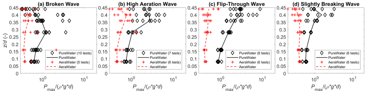
Figure 8: Impact pressures in pure and aerated water.
