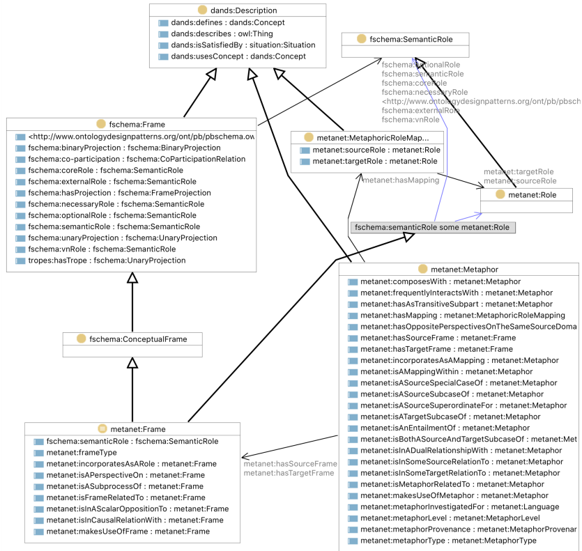
Fig. 2: A class-diagram profile for the OWL axiomatisation of Amnestic Forgery.
