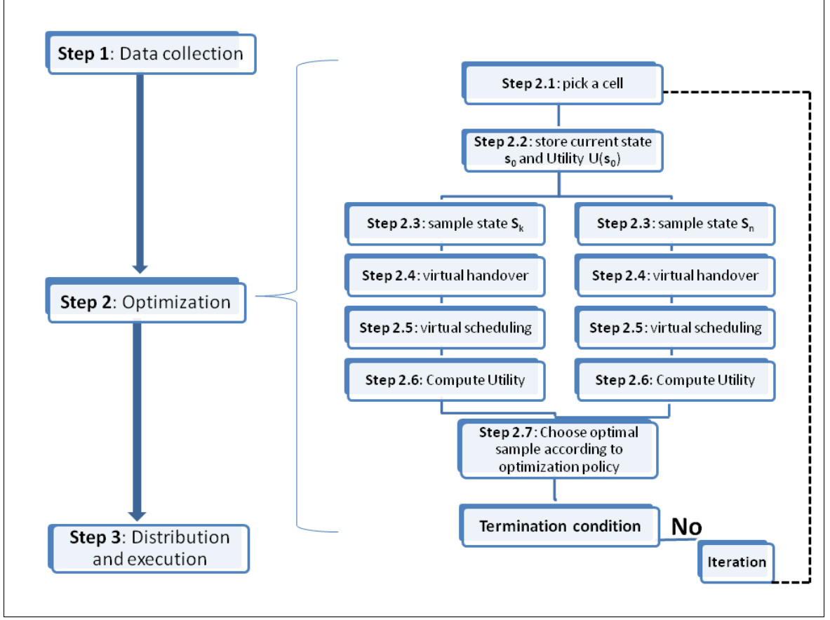
Figure 4.1: Framework overview.
