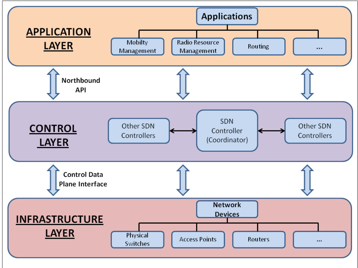
Figure 2.15: SDN architecture.
