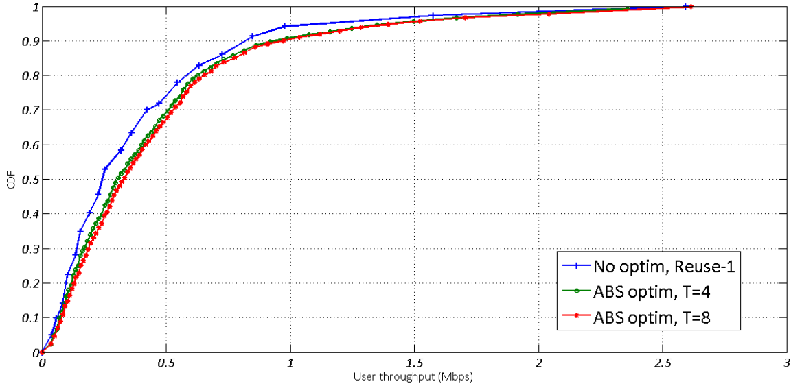
Figure 5.9: CDF user throughput (ABS Optim vs Reuse-1)- HetNets.
