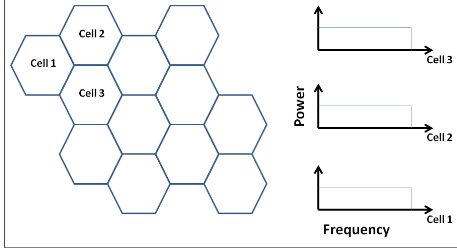
Figure 2.8: Frequency Reuse 1.
