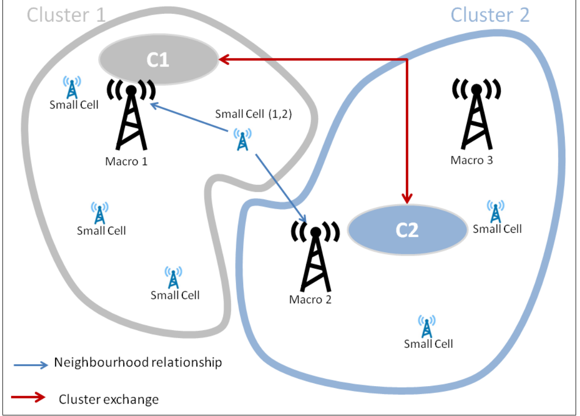
Figure 4.5: Clustering.
