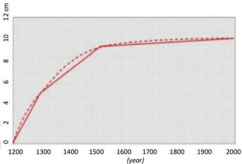
Figure 7. Graph of the hypothesized evolution of the main cracks on sides 1, 3, 5 of the dome, starting from its construction (at the end of XII century): The increasing trend has clearly decreased after the insertion of the two hoopings systems.
