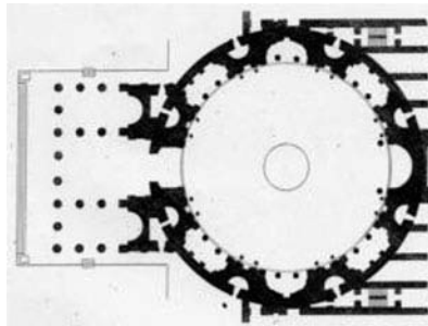
Figure 2. The perfect geometry of the Roman Pantheon, plan and section (Milani 1920). © [rightsholder]. Reproduced by permission of [rightsholder]. Permission to reuse must be obtained from the rightsholder.
