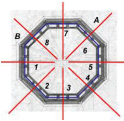
Figure 19. The crack pattern in Madonna dell'Umiltà dome: A (in red) and B (in blue).
