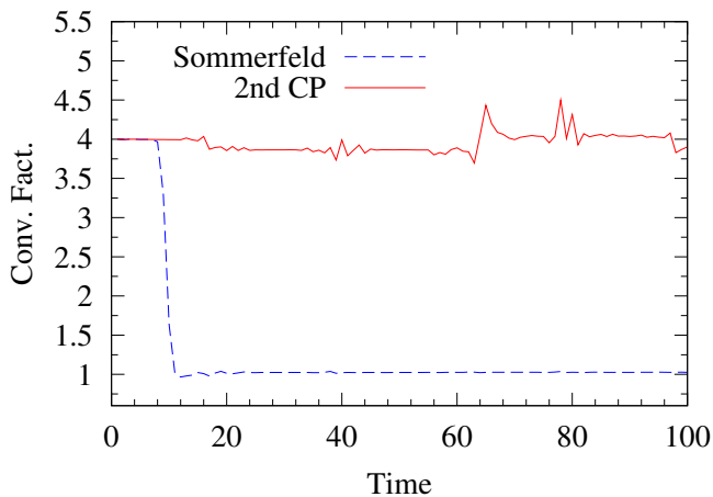
FIG. 5. Convergence factor in flat spacetime test. The self-convergence factor is computed from the 2-norms of three simulations at different resolutions and shown in time for 2nd order CPBCs and Sommerfeld BCs.
