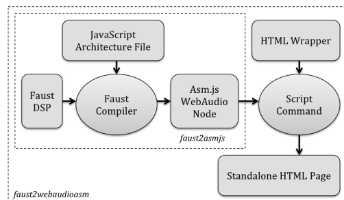
Figure 9: faust2asmjs and faust2webaudioasm compilation chains
