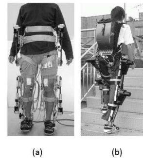
Fig. 6. HAL robotic exoskeleton, (a) the first prototype HAL-1, and (b) the second product HAL-3 [19].
