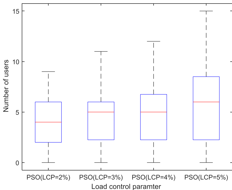
Fig. 6 Number of users per BS for different load control parameter. This figure shows the load per base station when the per base station biasing using particle swarm optimisation is implemented. It shows how particle swarm optimisation can control the number of users that are located at the cell expansion area
