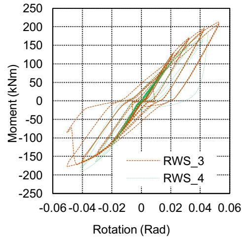
Figure 5 Hysteretic graph of RWS_3/RWS_4
