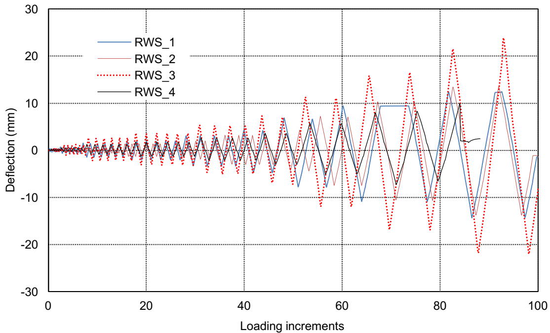
Figure 7 Vertical deflection across the 1 st web opening
