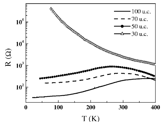
FIG. 4. Resistance versus temperature behavior for the four LSMO films on LAO substrates investigated in this paper.
