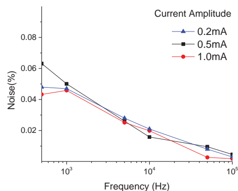
Figure 1: Noise levels, as a percentage of the mean voltage at the frequency of interest, measured across a 1k \Omega resistor over 1000 cycles.
