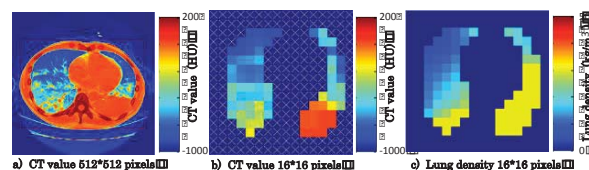
Figure 1: An example of comparison between CT values (HU) and Lung density ( \text{kg/m}^3 ) in a patient.
