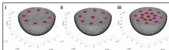
Figure 2: FEM meshes of 8 (i), 9 (ii), and 17(iii) electrode probe designs. The hemisphere represent the tissue volume being probed.
