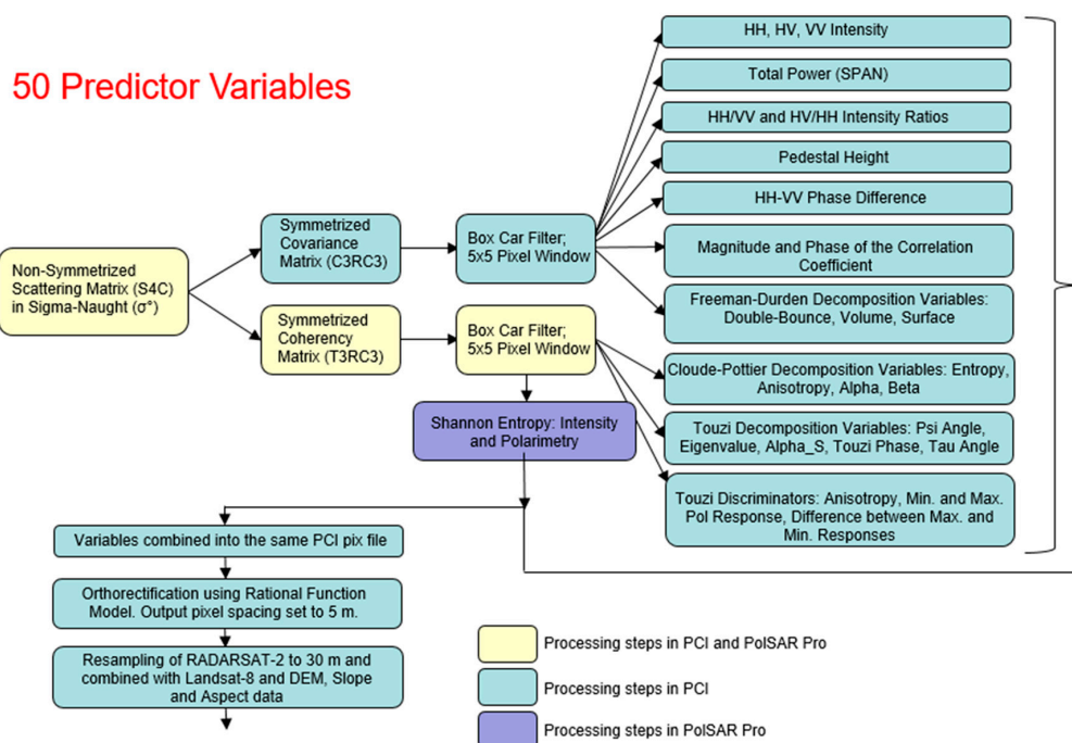
Figure 3. Processing steps used in PCI Geomatica 2015 and PolSAR Pro to generate the 50 predictor variables that were used in the RADARSAT-2 RF model (recreated after [50]).
