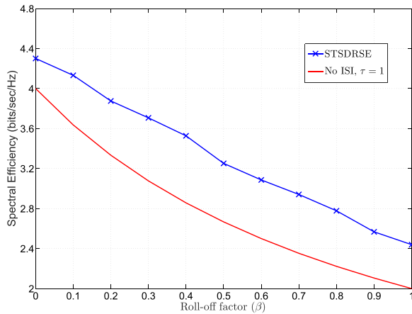
FIGURE 4. Spectral efficiency of 16-QAM FTN signaling as a function of \beta using the proposed STSDRSE at BER = 10^{-4} .
