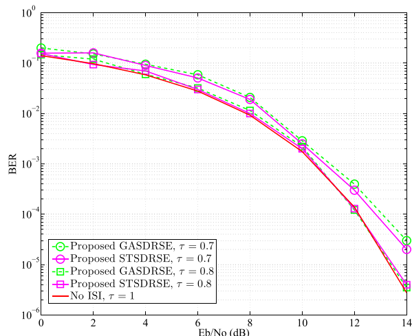
FIGURE 3. BER performance of 16-QAM FTN signaling as a function of E_b/N_0 for the proposed GASDRSE and STSDRSE techniques for \beta = 0.5 and \tau = 0.7 and 0.8 .
