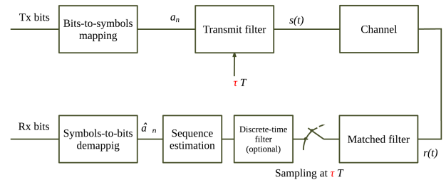
FIGURE 1. Block diagram of FTN signaling.
