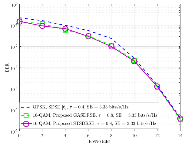
FIGURE 6. Performance comparison between 16-QAM FTN detection using the proposed GASDRSE and STSDRSE techniques and QPSK FTN signaling optimal detection using the sphere decoding in [6], for \beta = 0.5 and same spectral efficiency of 3.33 bits/s/Hz.
