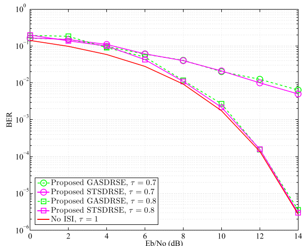
FIGURE 2. BER performance of 16-QAM FTN signaling as a function of E_b/N_0 for the proposed GASDRSE and STSDRSE techniques for \beta = 0.3 and \tau = 0.7 and 0.8 .
