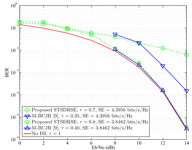
FIGURE 5. Performance comparison between 16-QAM FTN detection using the proposed STSDRSE technique and QPSK FTN signaling detection using the scheme in [9], for \beta = 0.3 and same spectral efficiencies of 4.3956 and 3.8462 bits/s/Hz.
