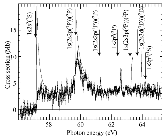
FIG. 1. Total double photodetachment cross section of \text{Li}^- giving rise to \text{Li}^+ in the vicinity of the 1s threshold. The solid curve is the R -matrix calculation and the dots with error bars are the experimental data normalized to the calculation at 62 eV. The arrows indicate neutral \text{Li} thresholds.
