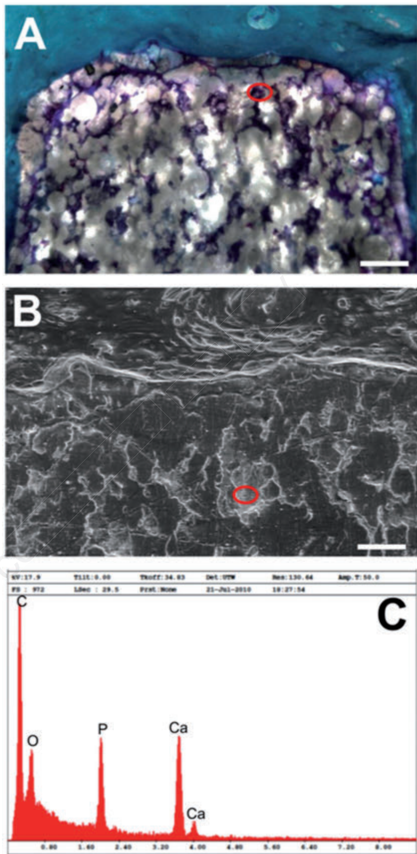
Figure 8. P cement, optical (A) and ESEM (B) microscopy at 12 months. The microanalysis of the sample (C) shows peaks of C, O, and significant peaks of P and Ca. Scale bars: A) 200 \mu\text{m} ; B) 100 \mu\text{m} .
