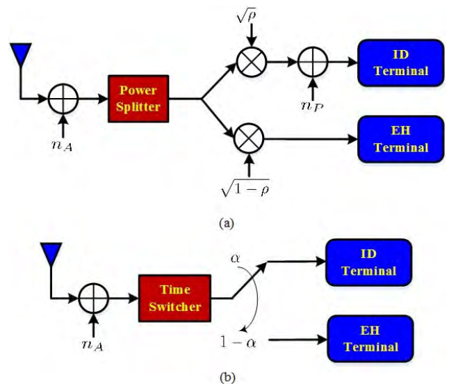
FIGURE 3. Receiver architecture for SWIPT with a single antenna. (a) Power-splitting mode; (b) time-switching mode.
