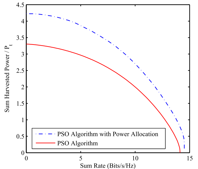
FIGURE 11. Power-rate tradeoffs of the PSO algorithms with and without power allocation in the 5-user IA-based network for wireless energy harvesting. Average received SNR is 10dB.
