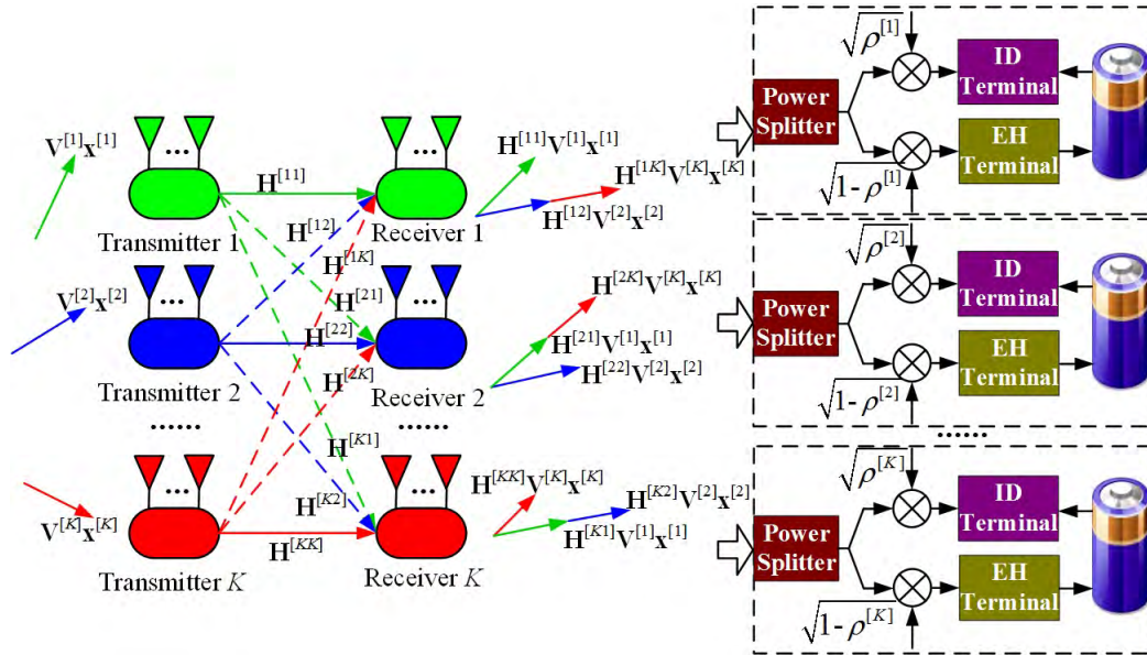
FIGURE 10. Demonstration of the IA-based wireless energy harvesting.
