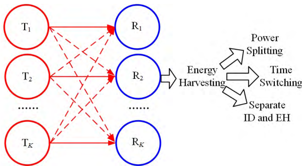
FIGURE 6. An interference network for wireless energy harvesting that exploits interference.
