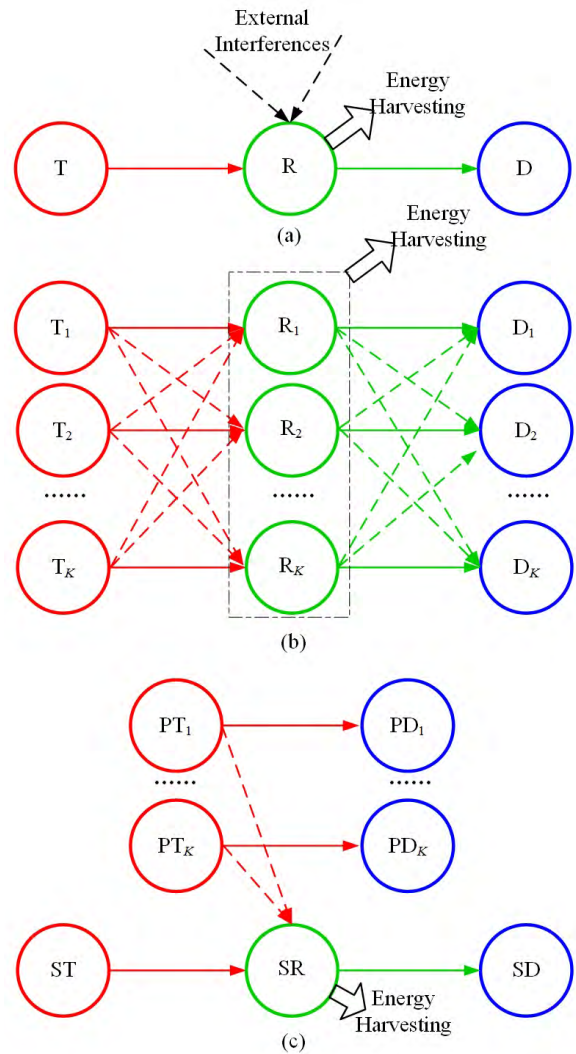
FIGURE 9. Three types of wireless energy harvesting in relay-based systems that exploit interference.
