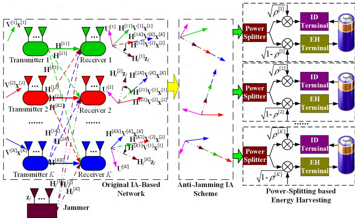
FIGURE 12. Demonstration of wireless energy harvesting in the anti-jamming IA network.
