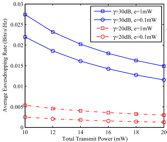
FIGURE 15. Comparison of the average eavesdropping rate in the anti-jamming AN scheme for wireless energy harvesting under different values of total transmit power, IT threshold \gamma and EH threshold e .
