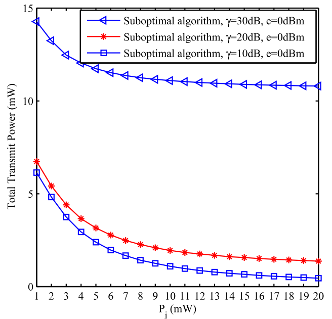
FIGURE 13. Comparison of the total transmit power of the proposed anti-jamming IA scheme with wireless energy harvesting when the transmit power of jammer and the threshold for IT \gamma are changing.
