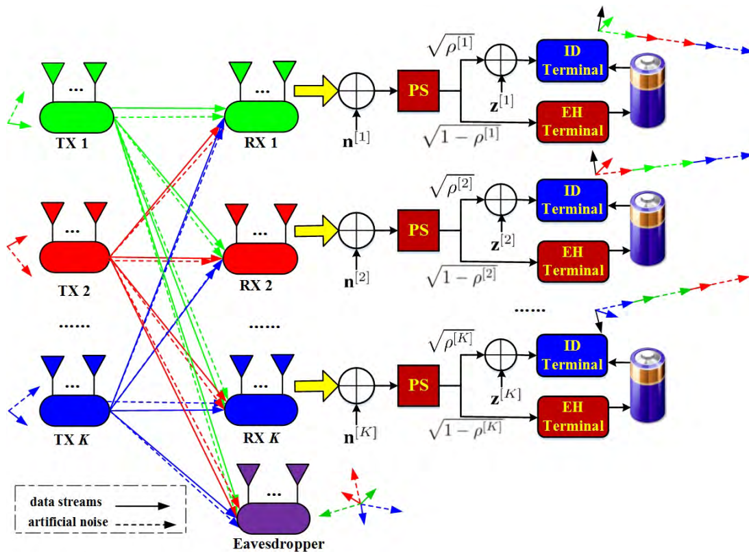
FIGURE 14. Demonstration of wireless energy harvesting in the anti-eavesdropping IA network with artificial noise.
