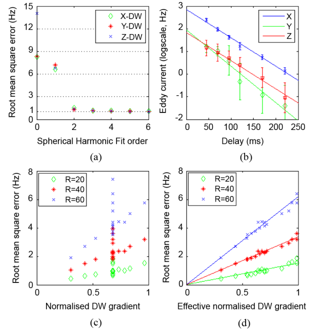
Fig. 2. Validation of model assumptions. The residual RMSE of the eddy current field, for each of the three diffusion-weighting gradients, b-value 2000 \text{ s/mm}^2 aligned along the principal axis, reduces with the order of the spherical harmonic fit (a). Image (b) shows the expected linear trend between the mean of the log(RMSE) as a function of delay. Images (c) and (d) plot the raw root mean square error of the eddy current field, aligned along the X-axis, from three surfaces of different radii (20, 40, and 60 mm) against the normalized diffusion-weighting gradient amplitude (c) and the effective normalized gradient amplitude (d) predicted by (1). Normalized diffusion-weighting gradient amplitude can only model protocols where the gradient shape, the TR or delay do not change; however applying linear response theory enables the model to be predictive of these changes to the protocol.
