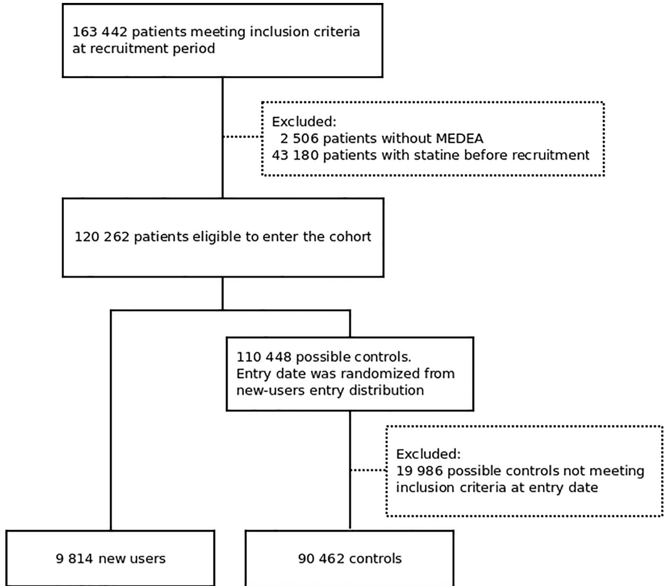
Fig 1. Study flowchart.
