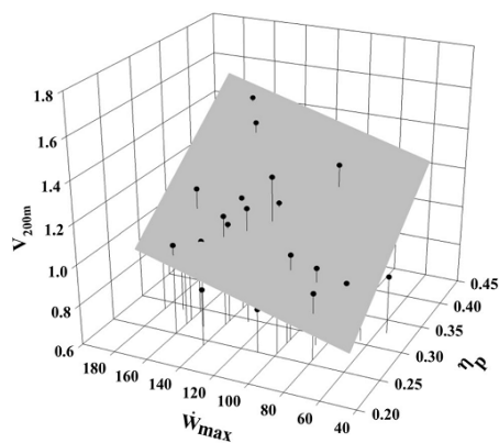
Fig. 4 The multiple linear regression between maximal power output ( \dot{W}_{\max} , dry-land test, W ), propelling efficiency ( \eta_p ) and swimming speed during the 200 m maximal trial ( V_{200 \text{ m}} , \text{m s}^{-1} ): about 75 % of the variability of V_{200 \text{ m}} can be explained by the variability of \dot{W}_{\max} and \eta_p ( R = 0.865 , P < 0.001 )
