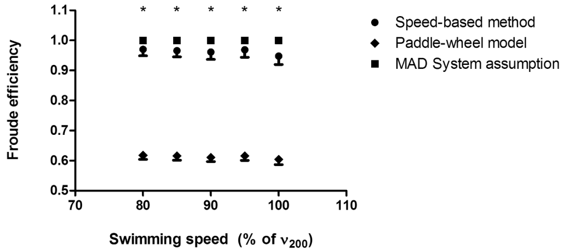
Figure 13. Values of stroke efficiency assessed in the MAD System condition by different methods in a range of speeds, from 80 to 100% of v_{200} .
