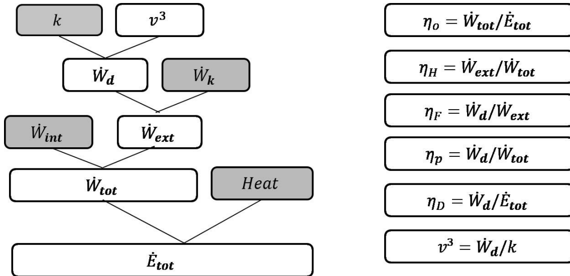
Figure 6. Useful and non-useful components of the cascade of efficiencies. \eta_o : overall efficiency; \eta_H : hydraulic efficiency; \eta_F : Froude efficiency; \eta_p : propelling efficiency; \eta_D : drag efficiency; \dot{E}_{tot} : total metabolic power input; \dot{W}_{tot} : total mechanical power output; \dot{W}_{int} : internal mechanical power; \dot{W}_{ext} : external mechanical power; \dot{W}_d : power needed to overcome drag (useful propulsive power); \dot{W}_k : power that does not contribute to generate propulsion; k : speed-specific drag coefficient; v : swimming speed.
