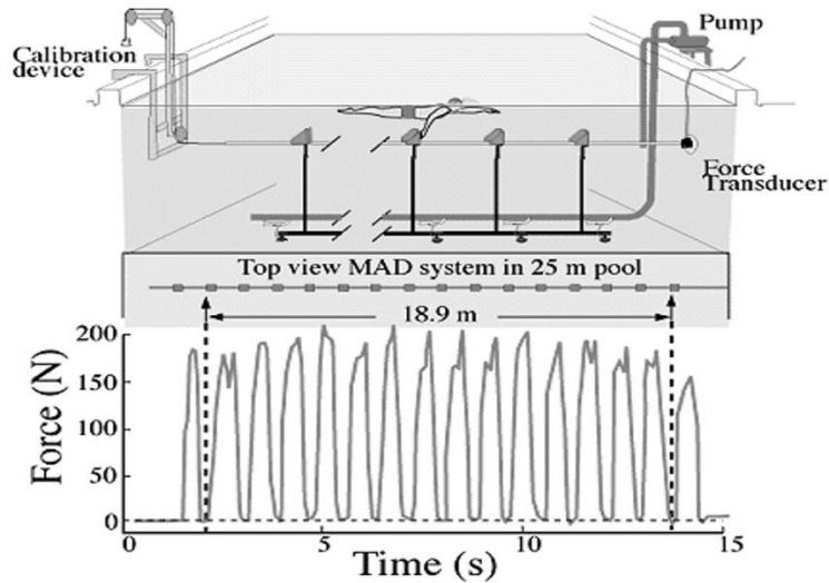
Figure 12. The structure of the MAD System. Forces were applied the push-off pads and assessed for each arm stroke by a force transducer (adapted from Toussaint et al., 1988).
