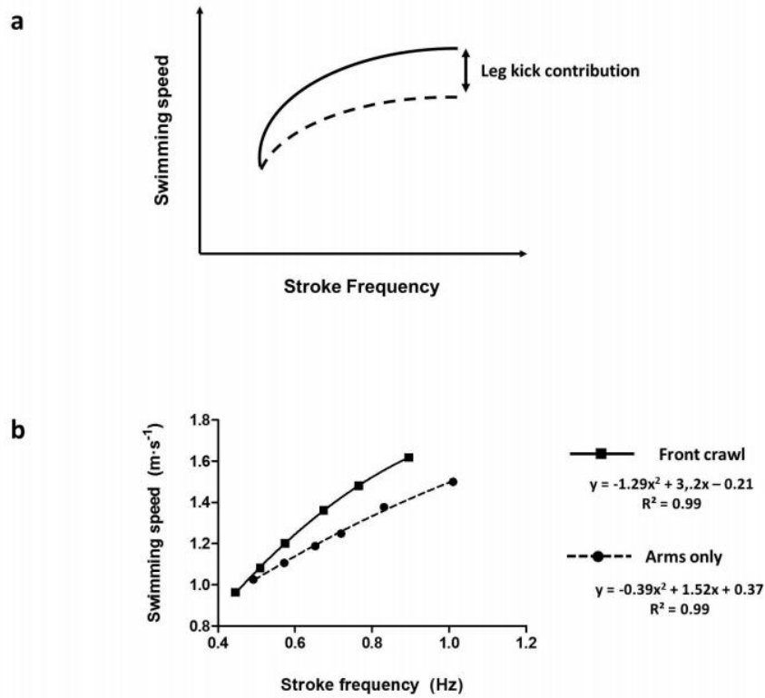
Figure 3. Stroke frequency ( SF ) vs. speed ( v ) relationship determined for the whole-body front crawl stroke ( FCS ) and swimming front crawl with the arms only ( SAO ) plotted to determine the contribution of the leg kick to forward speed ( LC ; the percentage difference in v between FCS and SAO at a given SF ).
