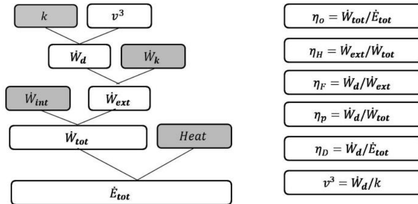
Figure 1. Useful and non-useful components of the cascade of efficiencies. \eta_o : overall efficiency; \eta_H : hydraulic efficiency; \eta_F : Froude efficiency; \eta_p : propelling efficiency; \eta_D : drag efficiency; \dot{E}_{tot} : total metabolic power input; \dot{W}_{tot} : total mechanical power output; \dot{W}_{int} : internal mechanical power; \dot{W}_{ext} : external mechanical power; \dot{W}_d : power needed to overcome drag (useful propulsive power); \dot{W}_k : power that does not contribute to generate propulsion; k : speed-specific drag coefficient; v : swimming speed.
