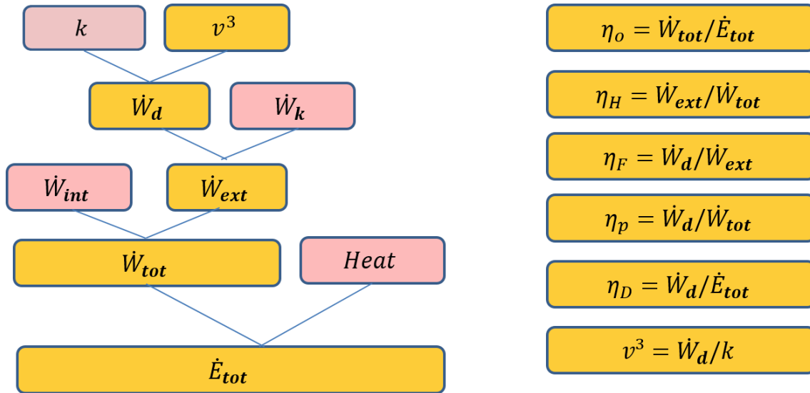
Figure 1. Cascade of fractionating energy expenditure rate into useful mechanical components (yellow) and not helpful (pink) in aquatic locomotion.
