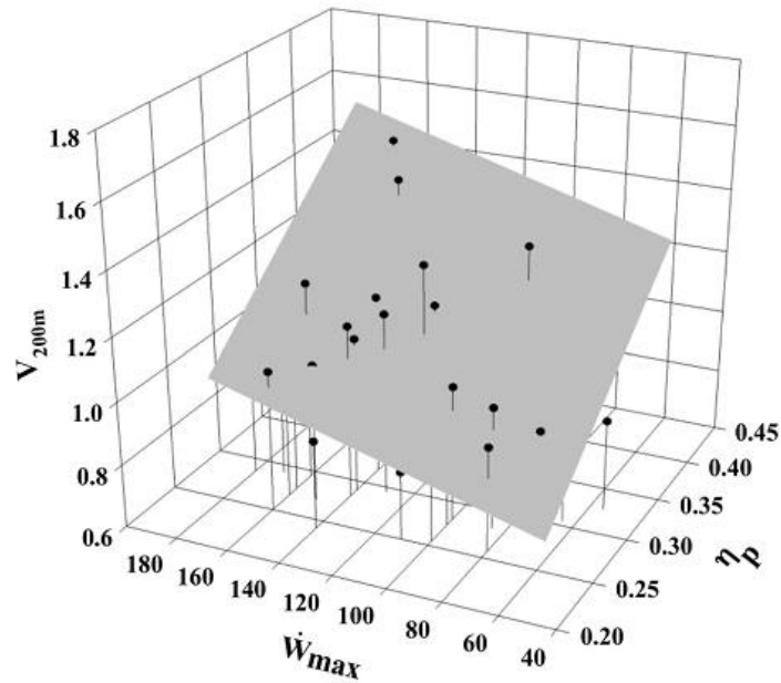
Figure 5. The multiple linear regression between maximal power output ( \dot{W}_{max} , dry-land test, W), propelling efficiency ( \eta_P ) and swimming speed during the 200 m maximal trial ( v_{200m} , m \cdot s^{-1} ): about 75 % of the variability of v_{200m} can be explained by the variability of \dot{W}_{max} and \eta_P ( R = 0.865 , P < 0.001 ).
