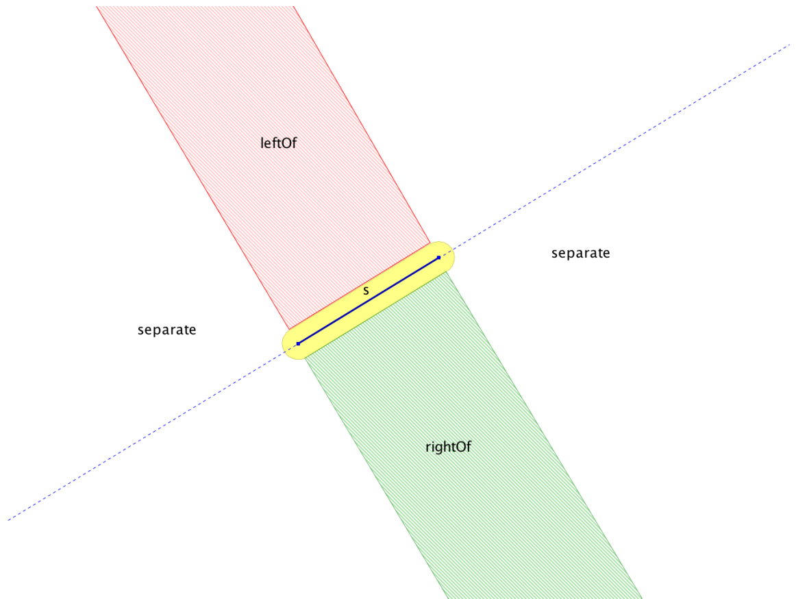
Figure 2: Regions defined by a segment s for the predicates leftOf(p, s) , rightOf(p, s) and separate(p, s) .
