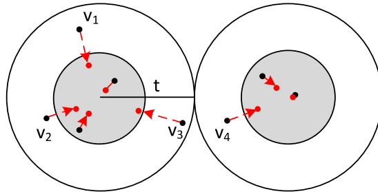
Figure 3: Example of application of the GATHERING procedure to two adjacent clusters. Vertices in the same cluster will be moved inside the gray region, called cluster kernel , in a position identified by the red points, which is proportional to their original distance from the cluster center.
