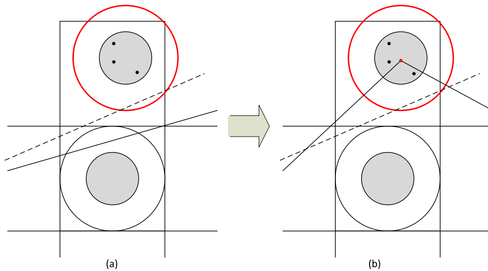
Figure 6: (a) Example of critical cluster: the solid edge e , produced at a certain stage of the TSR algorithm, passes through a cluster without passing through its kernel. The dashed line represents the original segment for the edge e . (b) Result of application of the REROUTE() procedure to edge e : since the original segment does not pass through the cluster but there exists a useful cluster such that e.os passes through it while e does not, case (b1) occurs and the edge e has to be splitted by adding a new vertex v at this cluster centroid.
