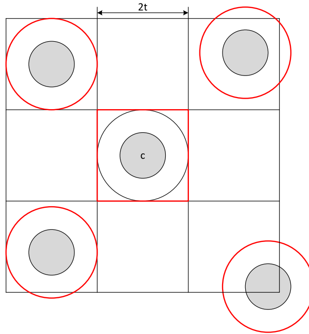
Figure 4: Example of frame for a cluster c placed at the center of the grid. The clusters composing the frame of c are those highlighted in red. Notice that a cluster belongs to the cluster frame even if it is not completely contained in a grid cell.
