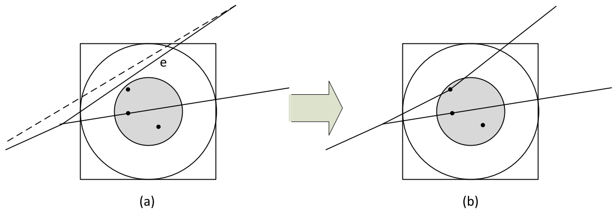
Figure 5: (a) Example of critical cluster: the solid edge e passes through a cluster without passing through its kernel. This produces a not-robust situation since the edge is neither well-separated nor coincident with the cluster vertices. The dashed line represents the original segment for the edge e . (b) Result of application of the REROUTE() procedure to edge e : since the original segment passes through the cluster, then case (a) occurs and the edge e has to be splitted by adding a new vertex v inside the cluster kernel.
