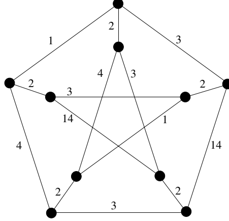
Figure 1: An excessive [4, 5] -factorization of the Petersen graph
