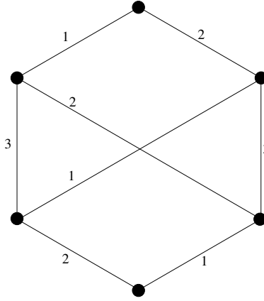
Figure 2: A graph which is not [2, 3] -coherent. As shown in the figure, \chi'_{[2, 3]} = 3 . It is easy to see that \chi'_{[2]}(G) = \chi'_{[3]}(G) = 4 .
