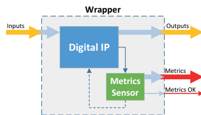
Fig. 1. Wrapping of digital IP and sensors to generate an “augmented” description.
