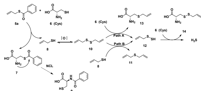
Scheme 3. Proposed Mechanism of H 2 S generation.
