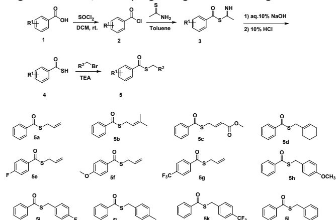
Scheme 2. Synthesis of thioester-based hydrogen sulfide donors 5a-l .
