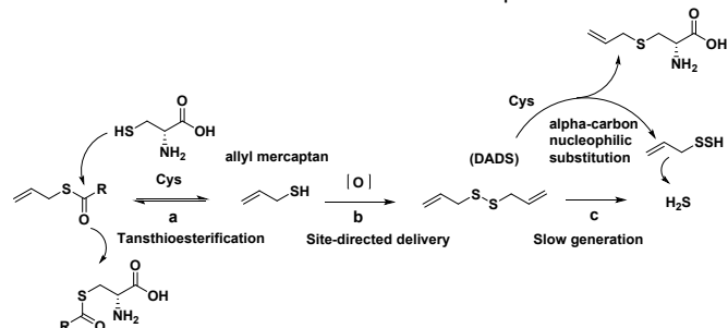
Scheme 1. Proposed controllable thioester-based hydrogen sulfide slow release donors.
