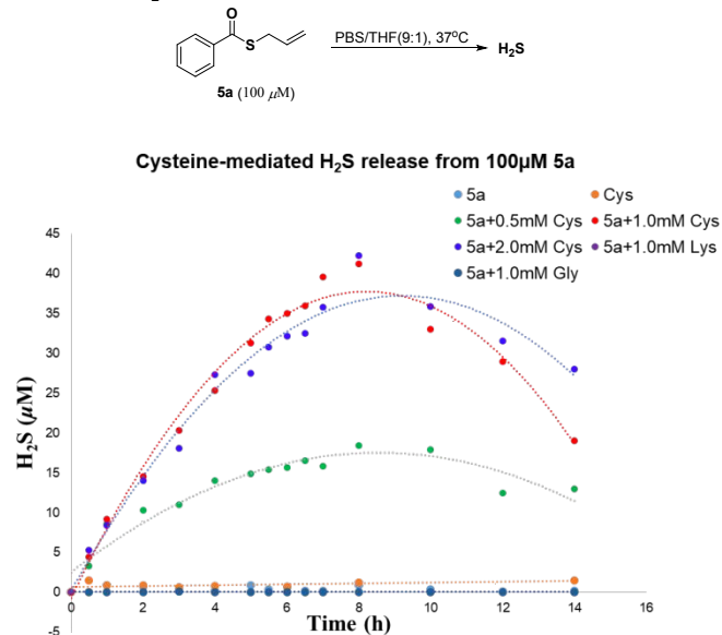
Figure 2. Cysteine mediated H 2 S release from compound 5a .
