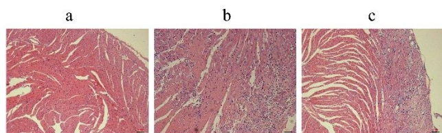
Figure 5. H&E staining was performed using heart sections to determine the morphological changes. (a) Normal group; (b) Model group; (c) Treated with 5e , 30 mg/kg/day. Scale bar: 10 \mu m.
