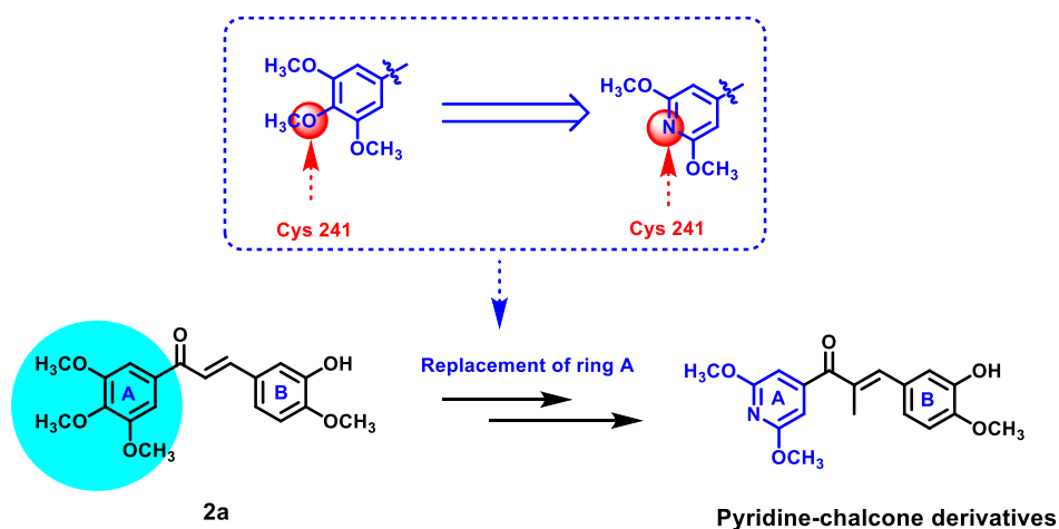
Figure 2. Design strategy of novel pyridine-chalcone derivatives.
