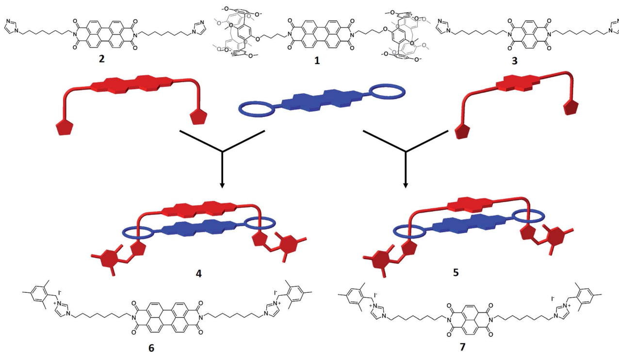
Fig. 1 PDI (1, 2) or NDI (3), containing components that are used to synthesise handcuff rotaxanes. Note the simple design of each component, either a bis-pillar[5]arene or bis-imidazole appended to an aromatic core. Handcuff formation is readily achieved through the formation of pseudo-rotaxanes between imidazole and pillar[5]arene moieties followed by stoppering through reaction of the imidazole groups and benzyl iodides. Model bis-imidazolium rods, 6 and 7, are studied for comparison.
