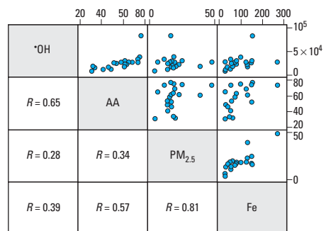
Figure 1. Scatter plot and Pearson correlation of annual mean \cdot\text{OH} , AA depletion rates, PM 2.5 total mass, and Fe mass concentration (units as in Table 1).
