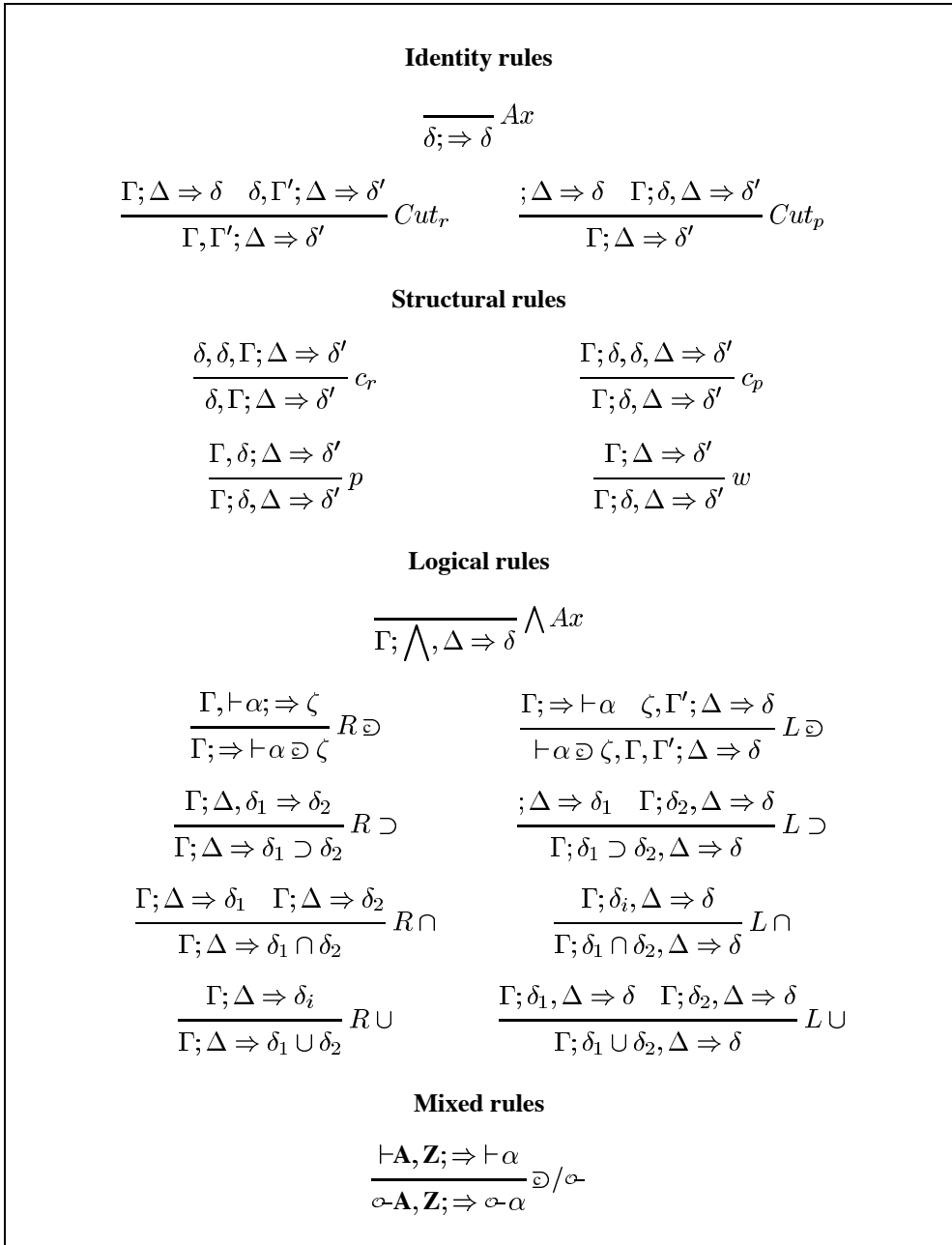
FIGURE 2. The sequent calculus ILP
