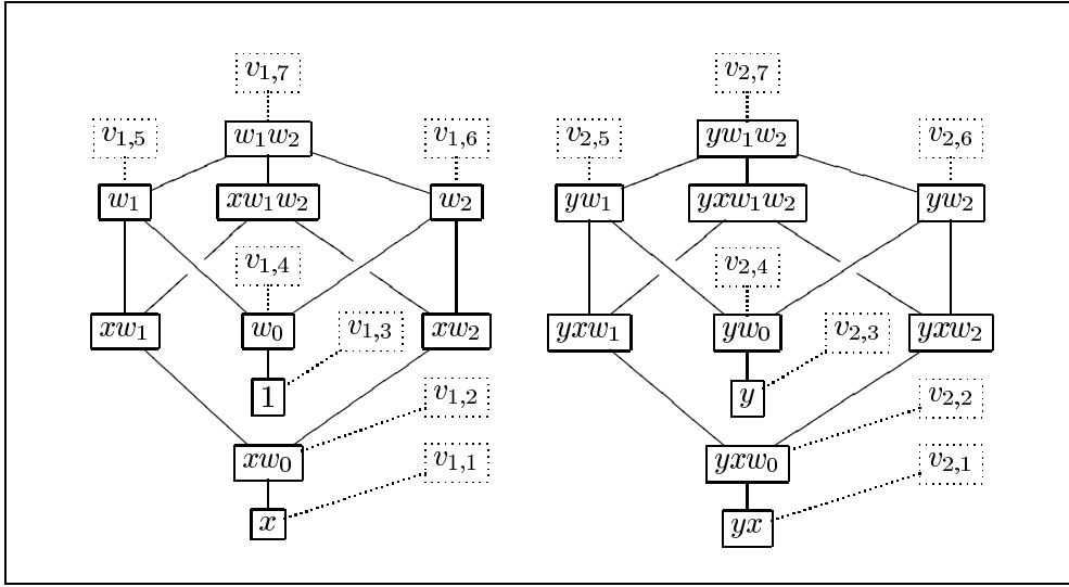
FIGURE 5. Example of a Kripke frame
