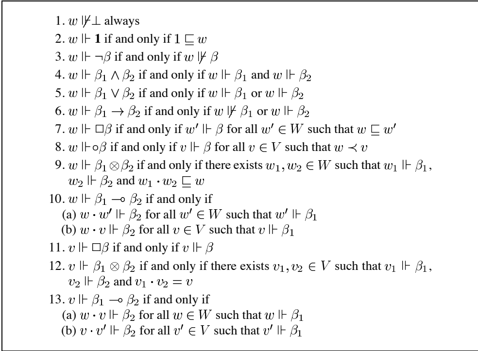
FIGURE 3. The forcing relation \vdash for extended radical formulas
