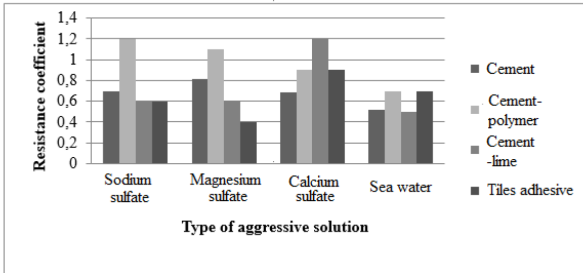
Fig. 1. Coefficient of corrosion resistance of dry building mixtures at the age of 180 days.
