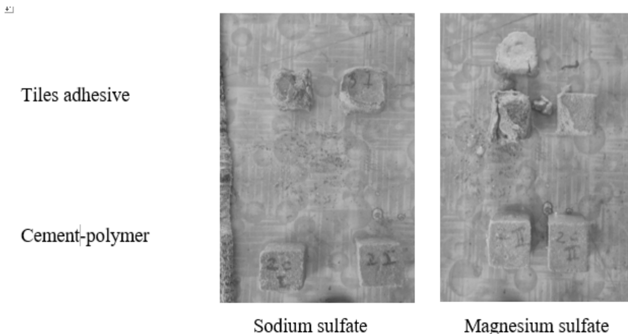
Fig. 2. Appearance of adhesive samples for tile and cement-polymer plaster after 180 days hardening in solutions of sodium sulfate and magnesium sulfate
